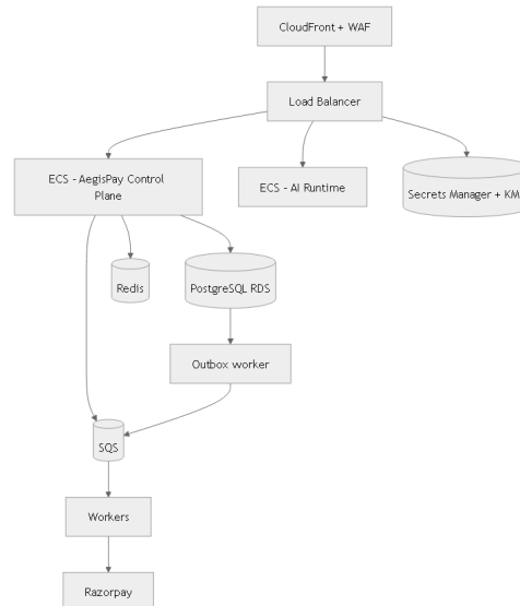
Figure 14 — Two ECS services, managed data, one queue
