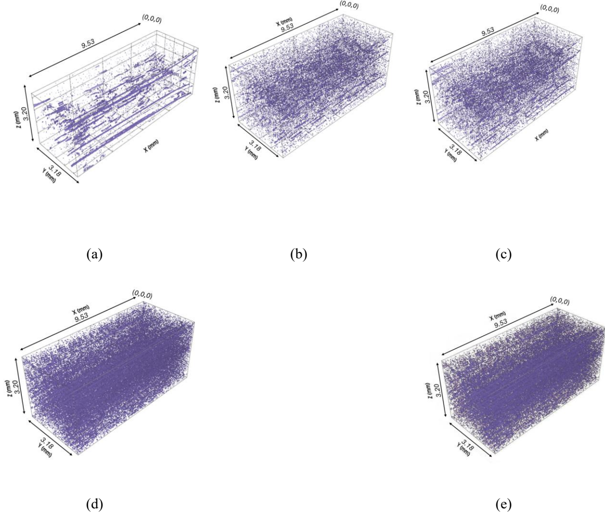
Figure 4.7 : Volumetric representation of raster voids in 3D-printed HDPE-HGM syntactic foams at varying infill densities and Compositions: (a) 100 % Comp. A, (b) 90 % Comp. B, (c) 80 % Comp. A, (d) 70 % Comp. B, and (e) 60 % Comp. A
