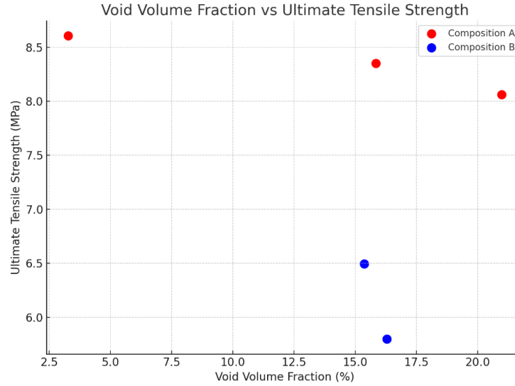
Figure 4.13 : The relationship between VF_{void} and UTS for all samples with varying infill densities and Comp. A and B. Red markers indicate samples with Comp. A, and blue markers represent Comp. B. A clear inverse trend is observed, with Comp. A maintaining higher tensile strength across a broader range of VF_{void} , highlighting the role of microstructural characteristics in governing mechanical performance.
