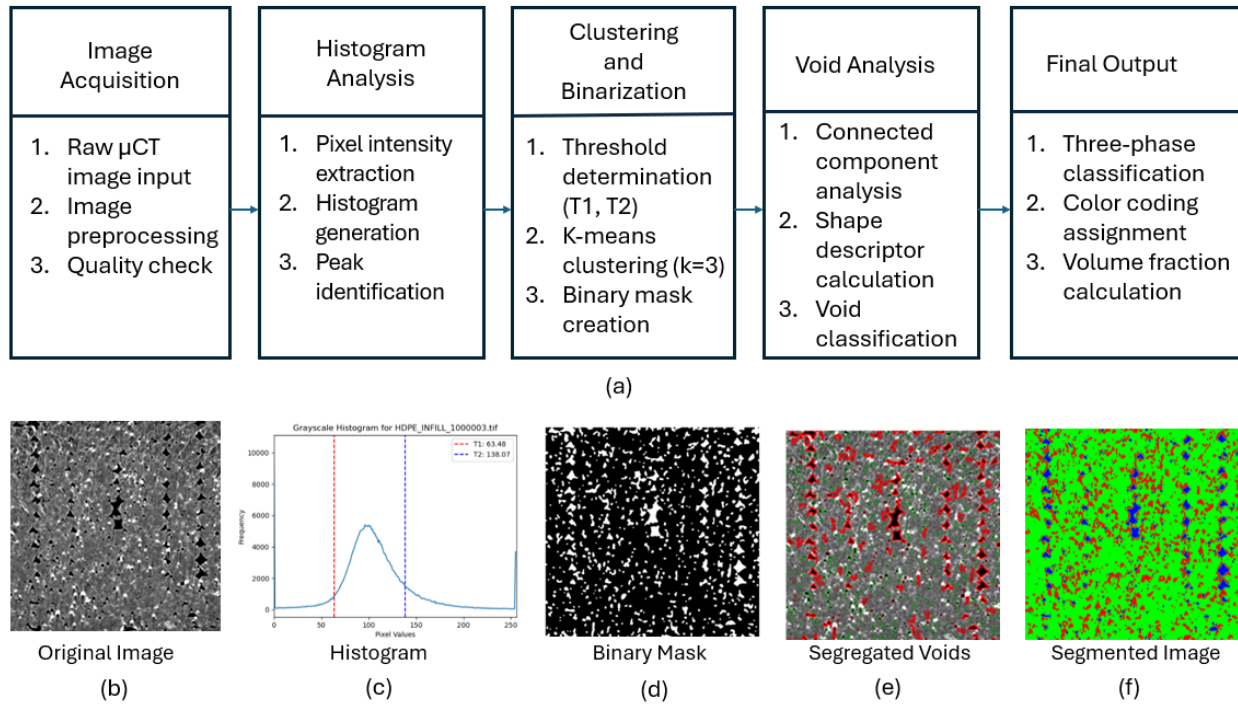
Figure 4.2 : Image segmentation methodology: (a) Complete processing workflow organized into five analysis stages, each corresponding to representative results shown in (b-f); (b) original \mu CT slice; (c) intensity histogram analysis; (d) binary mask generation; (e) void segregation; (f) three-phase segmented output.
