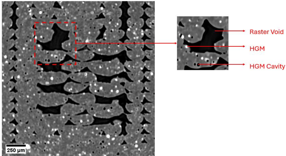
Figure 4.1 : Micro-CT image of HDPE – HGM Syntactic foam 100 % Infill Component A showing HGM in matrix material, highlighting raster voids, HGM particles, and HGM cavities.
