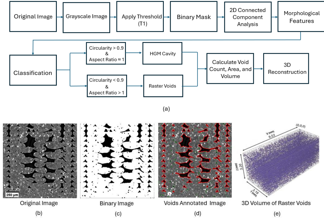
Figure 4.6 : Void classification and quantification workflow in 3D-printed syntactic foams: (a) Processing flowchart showing the sequential steps from original image through morphological analysis to final classification and 3D reconstruction; (b-e) Representative results demonstrating void identification: (b) original \mu CT slice; (c) binary mask generated using threshold T1; (d) annotated void classification showing raster voids in red and HGM cavities in green; (e) 3D volume reconstruction of classified void structures
