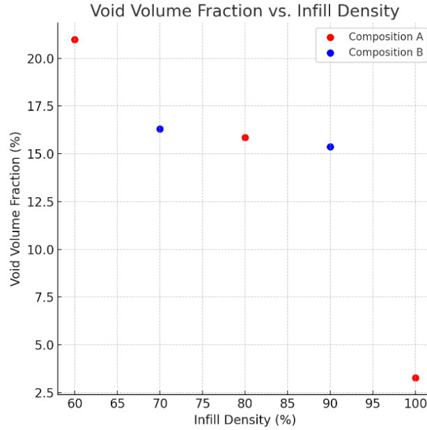
Figure 4.12 : Relationship between infill density and VF_{\text{void}} in HDPE-HGM syntactic foams, highlighting the differences between Comp. A (red) and Comp. B (blue). Lower infill densities correspond to higher void content
