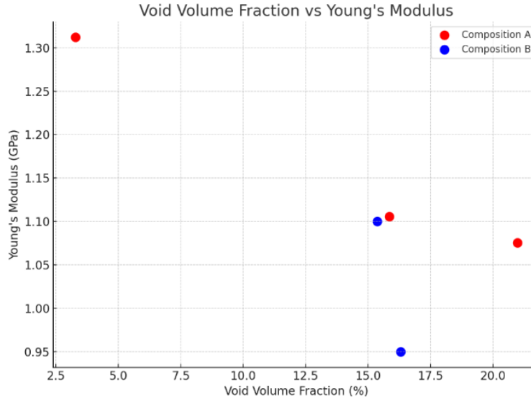
Figure 4.14 : Relationship between VF_{\text{void}} and Young's modulus for Comp. A and B. Red markers represent Comp. A and blue markers indicate Comp. B. A strong inverse relationship is evident, with Comp. A, maintaining higher stiffness over a broader VF_{\text{void}} range, indicating greater resistance to porosity-induced degradation.
