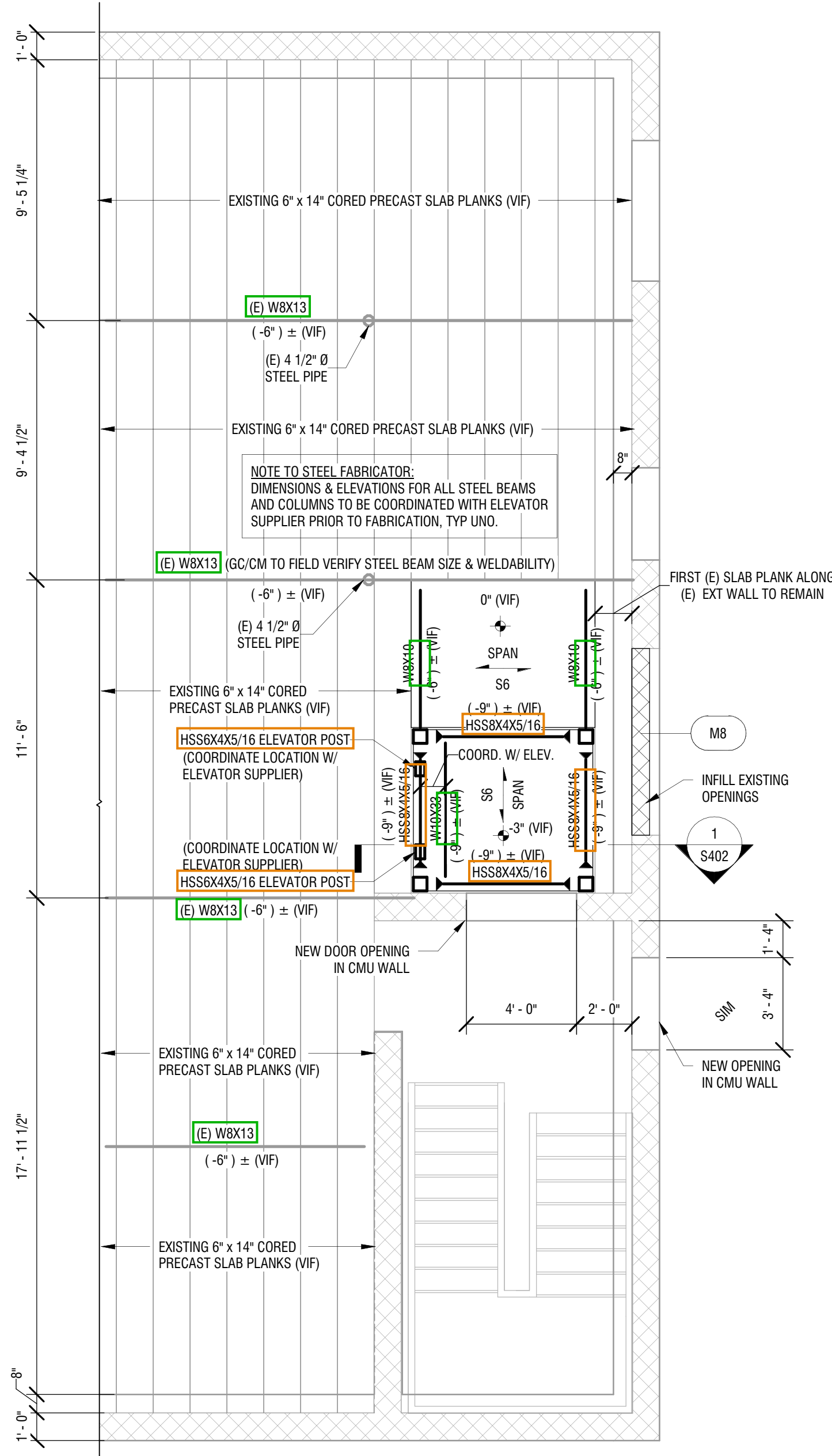
2 LEVEL 1 FRAMING PLAN- ALTERNATE #1 1/4" = 1'-0"
