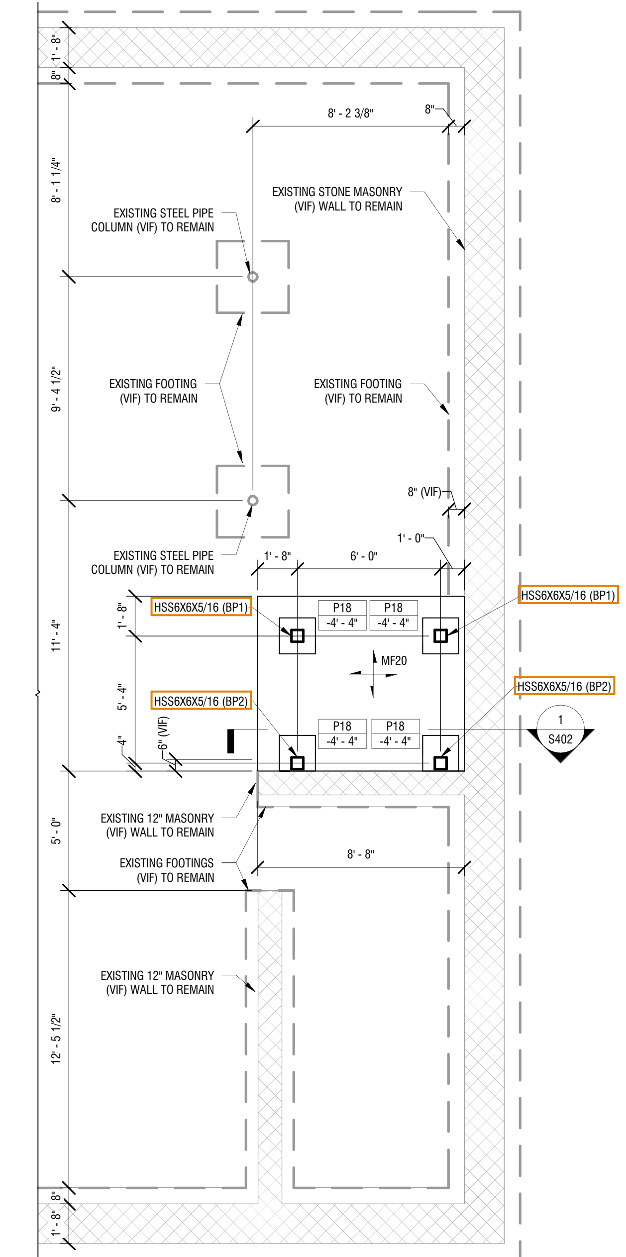
1 FOUNDATION PLAN- ALTERNATE #1 1/4" = 1'-0"
