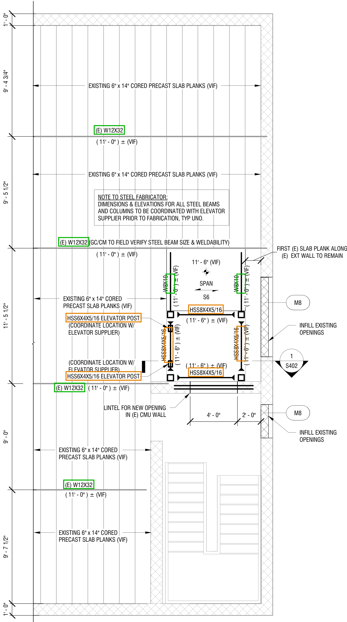
3 LEVEL 2 FRAMING PLAN- ALTERNATE #1 1/4" = 1'-0"
