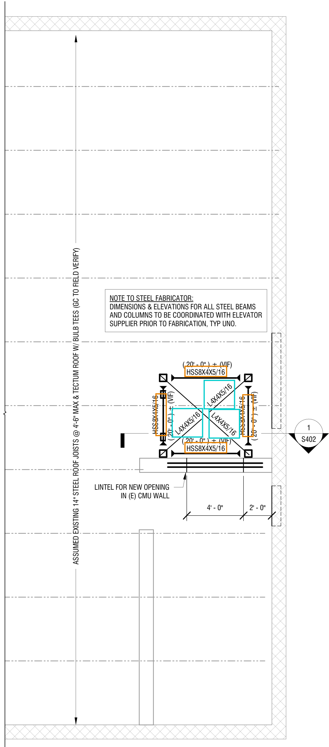
4 ROOF FRAMING PLAN- ALTERNATE #1 1/4" = 1'-0"
