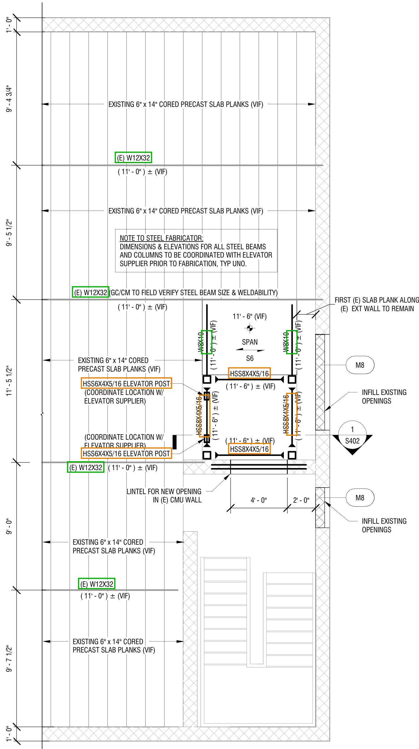
3 LEVEL 2 FRAMING PLAN- ALTERNATE #1 1/4" = 1'-0"
