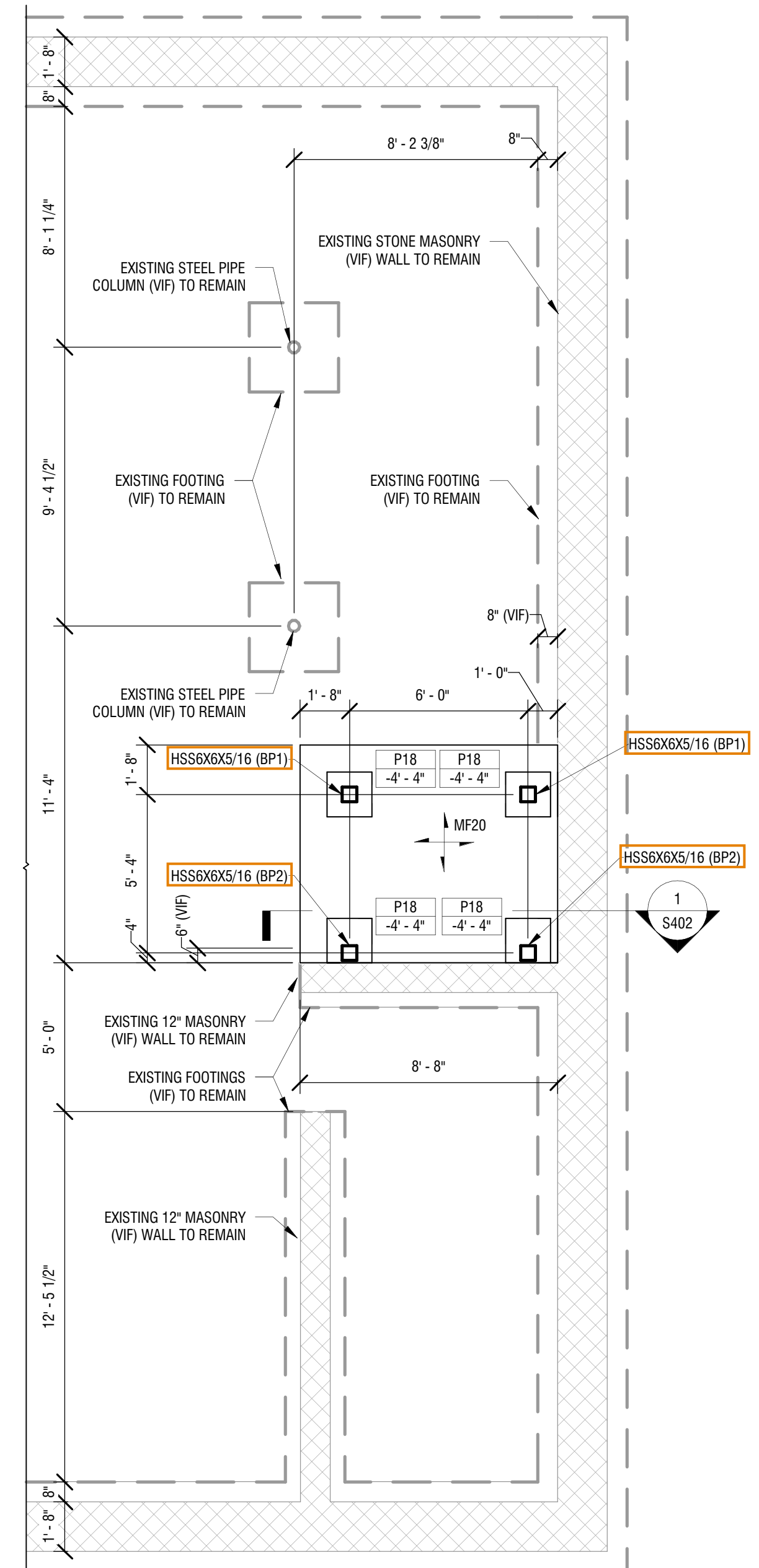
1 FOUNDATION PLAN- ALTERNATE #1 1/4" = 1'-0"
