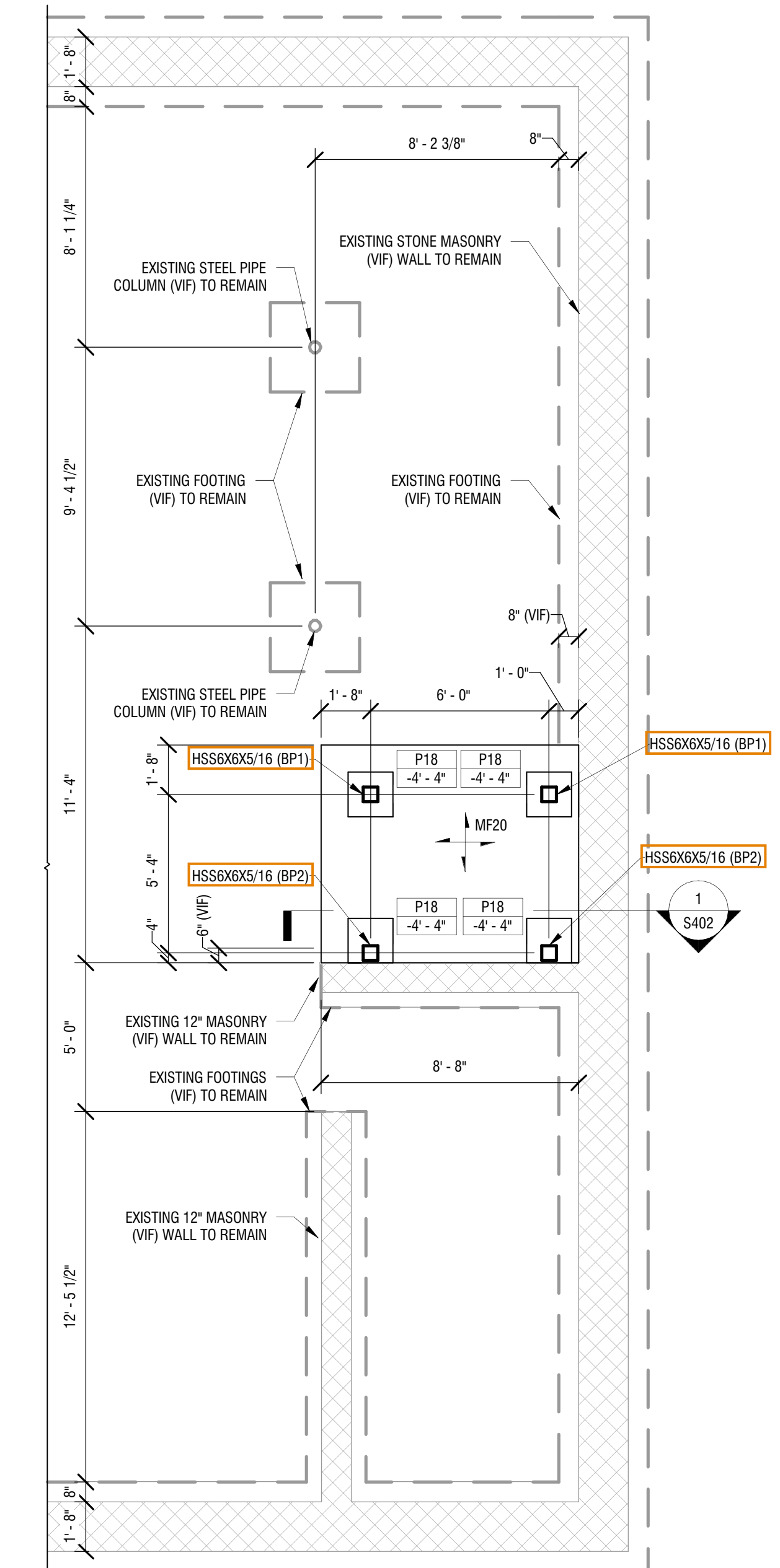
1 S401 1/4" = 1'-0"
