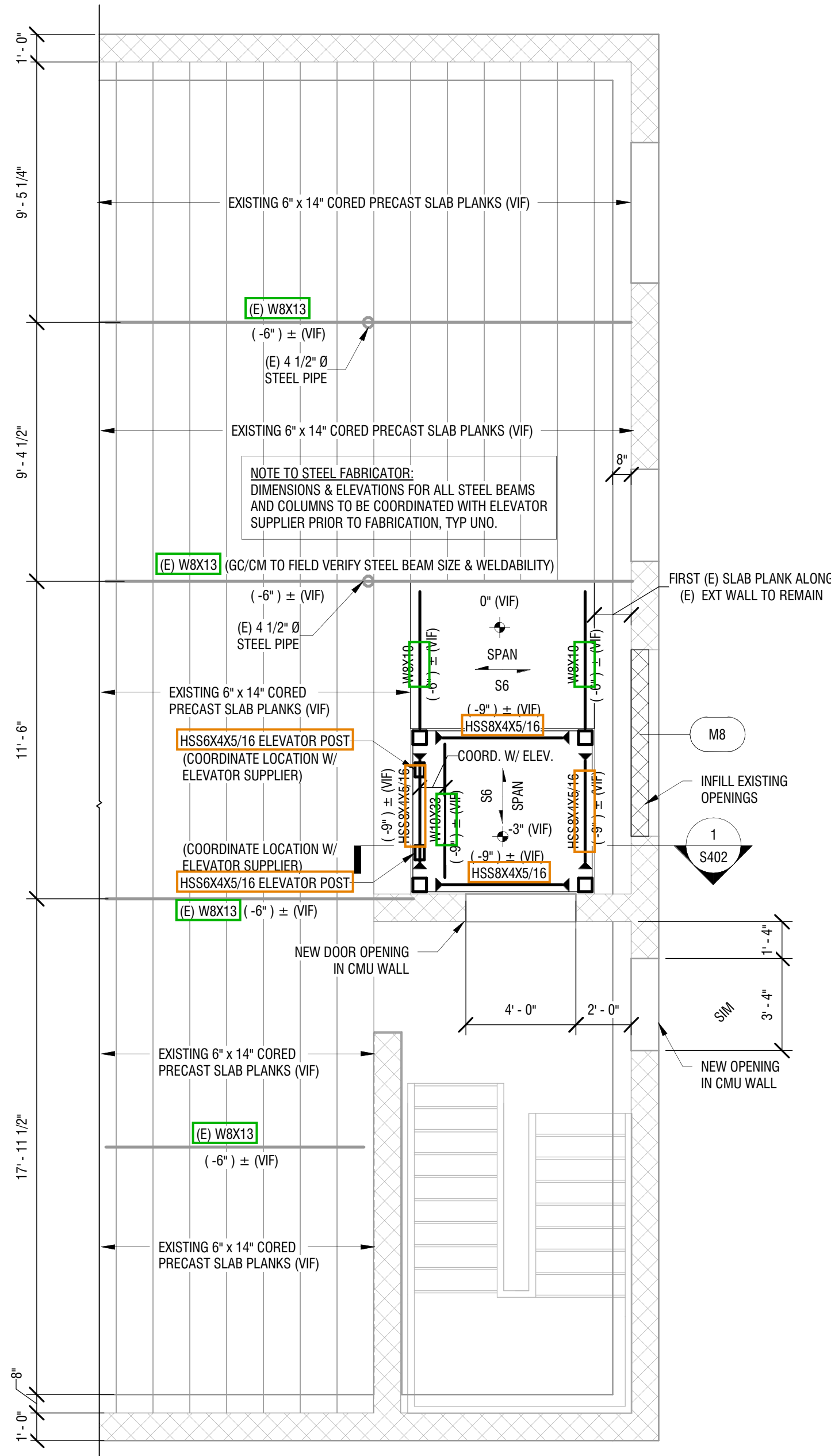
2 S401 1/4" = 1'-0"
