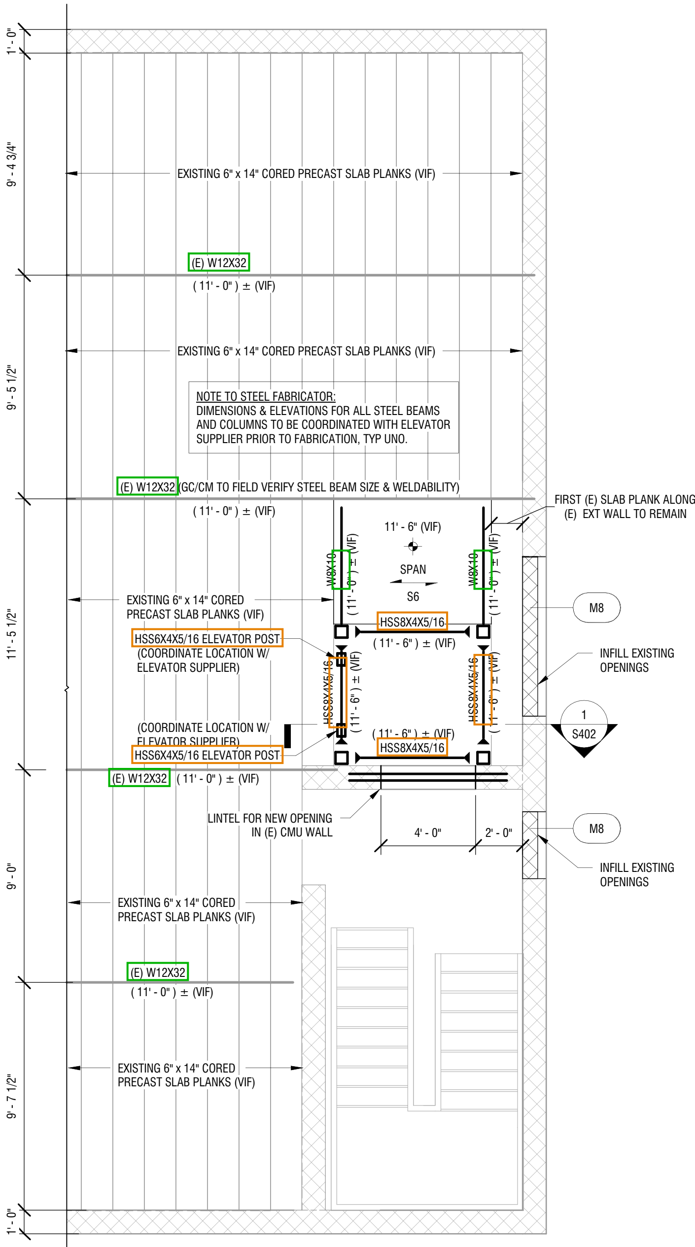
3 S401 1/4" = 1'-0"
