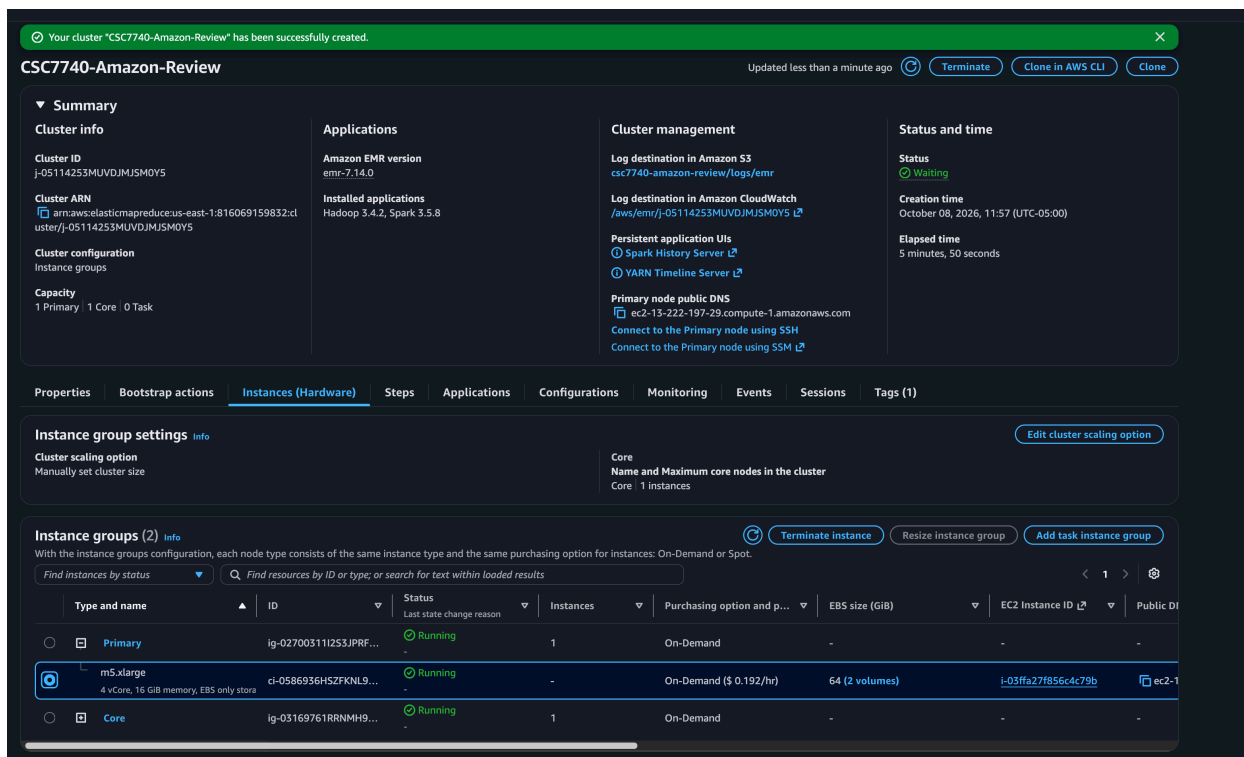
Figure 1. AWS EMR cluster j-05114253MUVDJMJS0Y5 in the Waiting state after successful creation. The console shows EMR 7.14.0, Spark 3.5.8, Hadoop 3.4.2, and the initial one-primary/one-core configuration.
