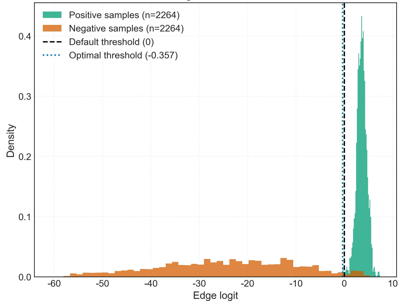
Logit distribution
