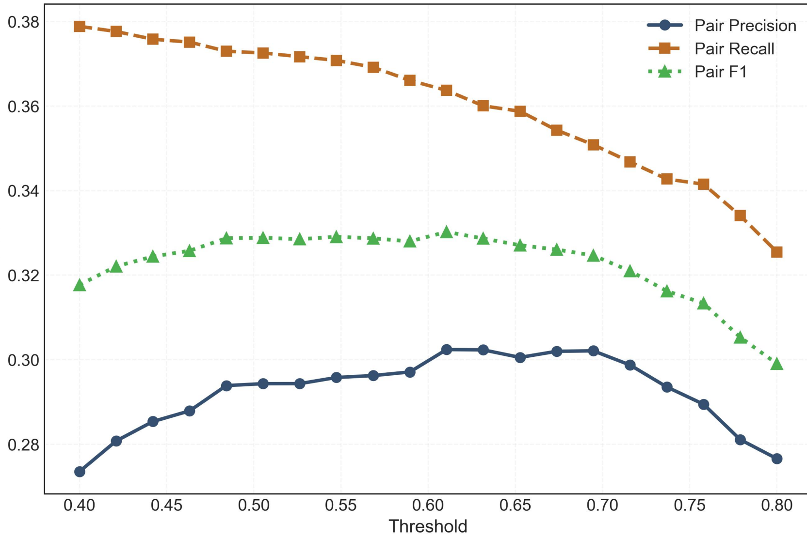
Pair-level Association Metrics
