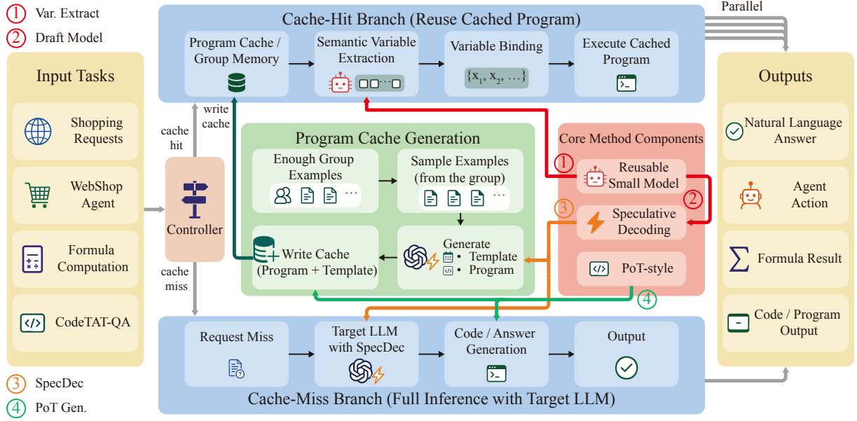
Figure 1: Overview of the proposed inference framework. The numbered arrows denote: (1) semantic variable extraction by the reusable small model, (2) the same small model as the speculative drafter, (3) SpecDec-accelerated target-LLM calls, and (4) PoT-style program generation for answers and cache construction.
