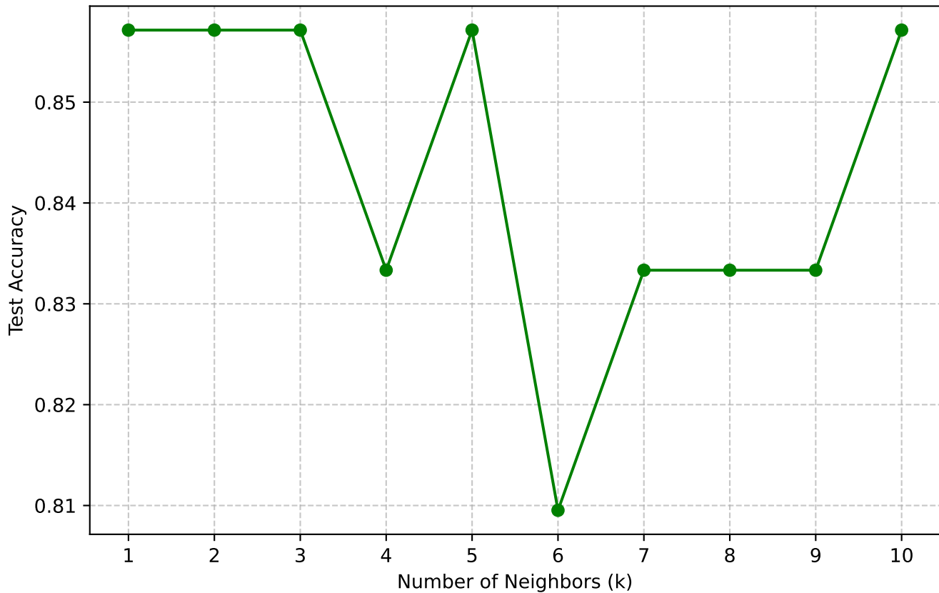
Scikit-Learn KNN Accuracy vs. k (Wheat Dataset)
