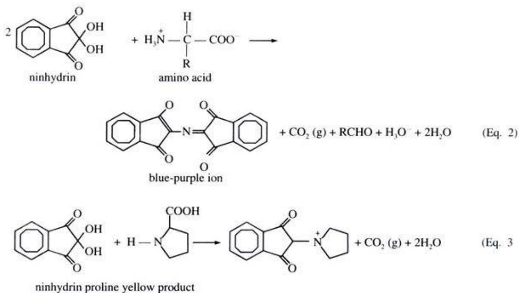
Figure 5 Original course reaction diagram: follow the amino-acid carbon skeleton and the colored product. The diagram supplies the chemistry; the two teacher versions differ in heating duration.
