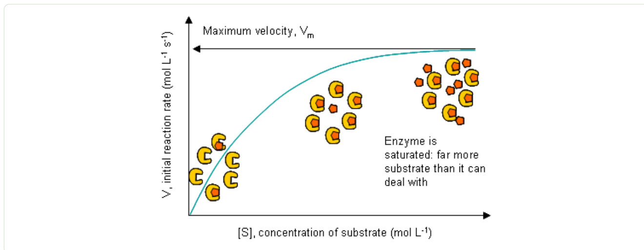
Figure 7 Original course saturation graph: the plateau reflects a finite enzyme catalytic capacity, not disappearance of substrate from the graph.
