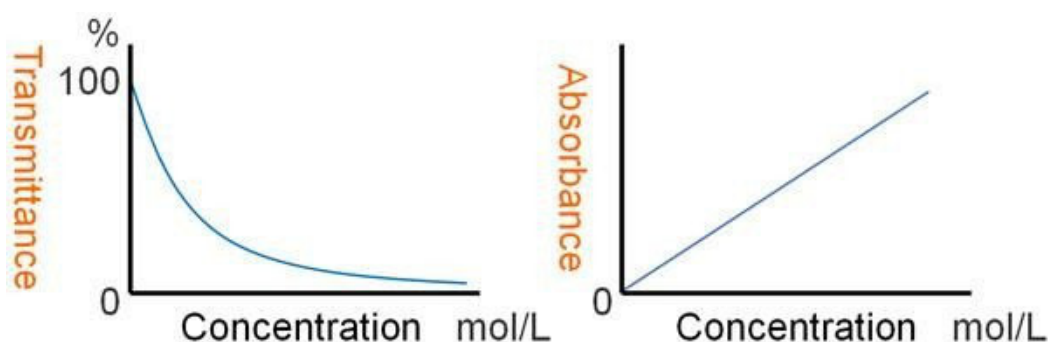
Figure 4 The source curves contrast exponential loss of transmittance with linear increase of absorbance as concentration rises. This is why calibration ordinarily uses absorbance rather than percent transmittance.
