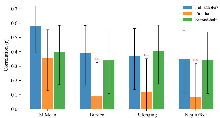
Figure 9: Temporal split validation. Adapters trained on the first or second half of each participant’s messages are compared to full adapters. Error bars indicate 95% CIs (Fisher z ). SI prediction is preserved across both splits, but construct-specific predictions (burden, belonging, negative affect) are recovered only by second-half adapters. n.s. = not significant.
