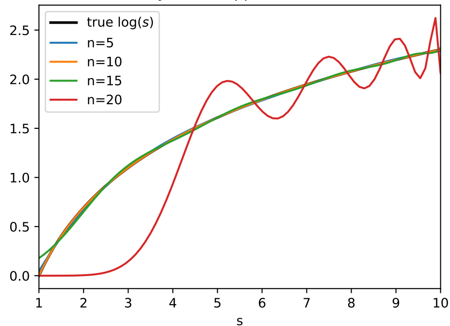
Polynomial approximations
