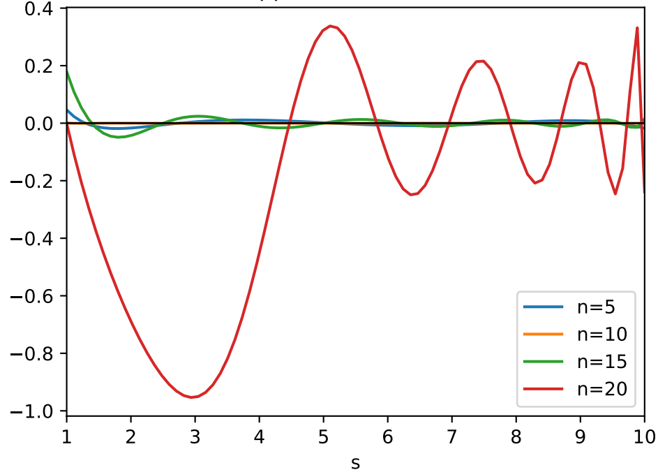
Approximation error
