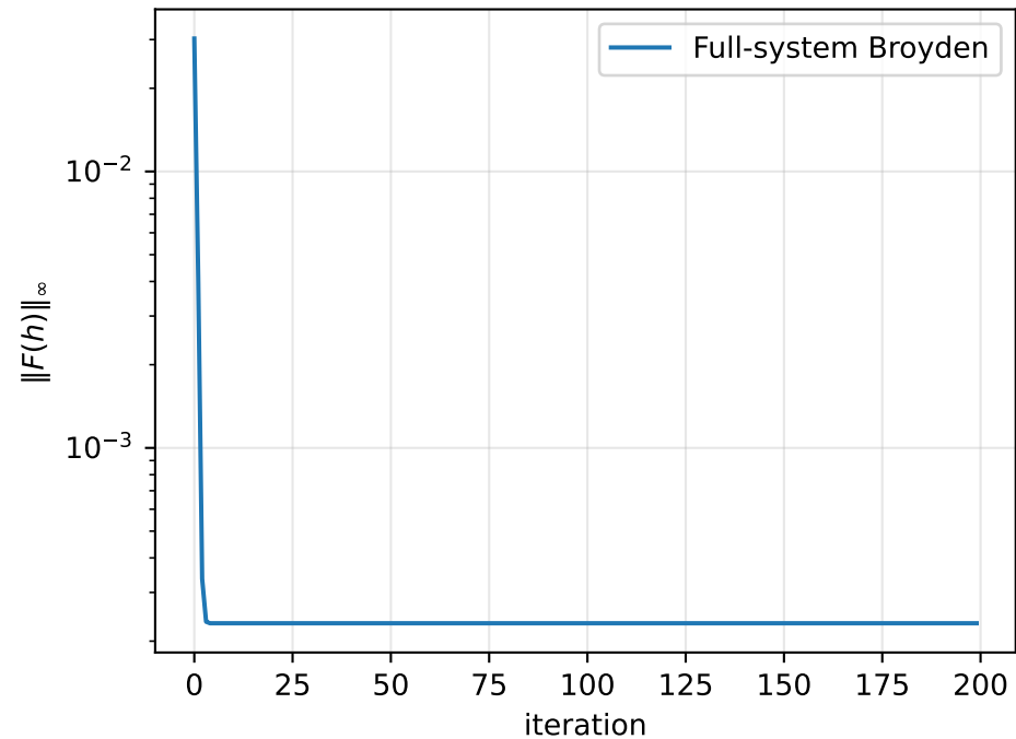
Broyden (full system)
