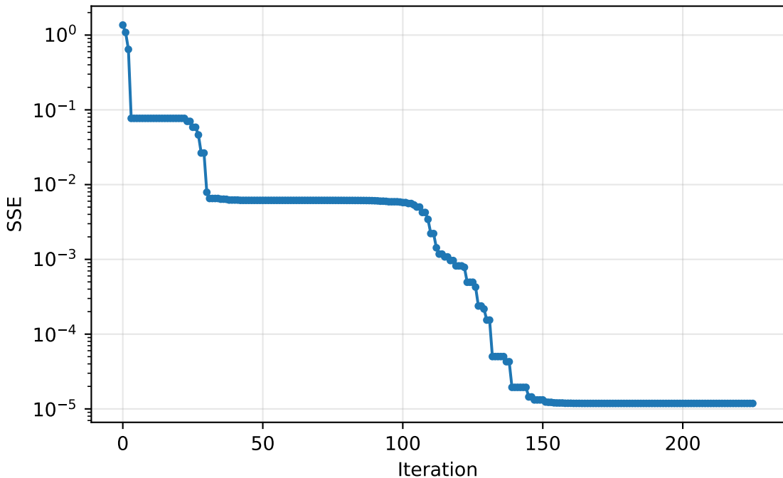
Nelder-Mead: SSE at each iteration
