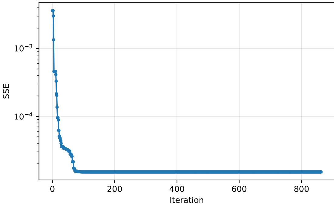
Nelder-Mead (jump-diffusion): SSE at each iteration
