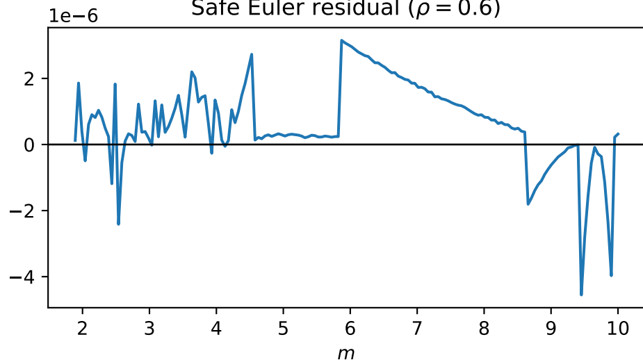
Safe Euler residual ( \rho = 0.6 )
