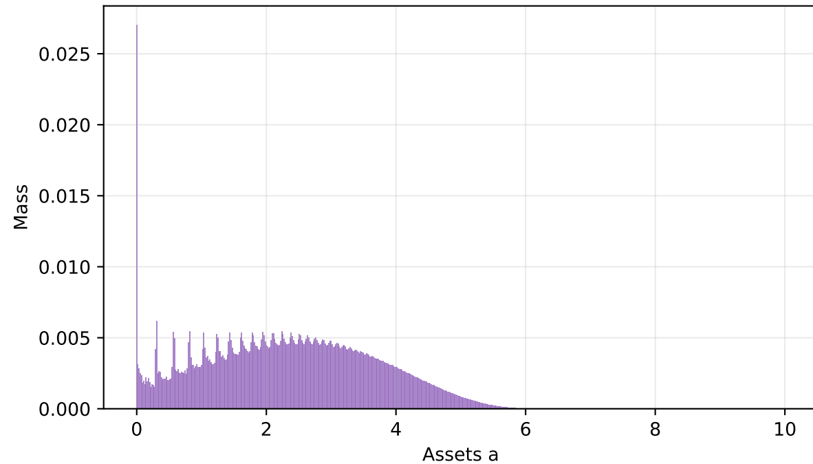
Ergodic Distribution (whole)
