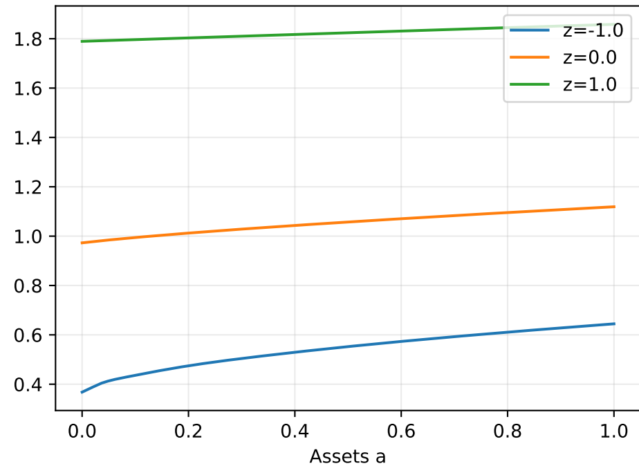
Consumption c(a,z) (spline-smooth)
