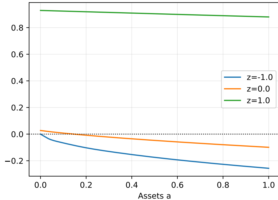
Savings a'(a,z) - a (spline-smooth)
