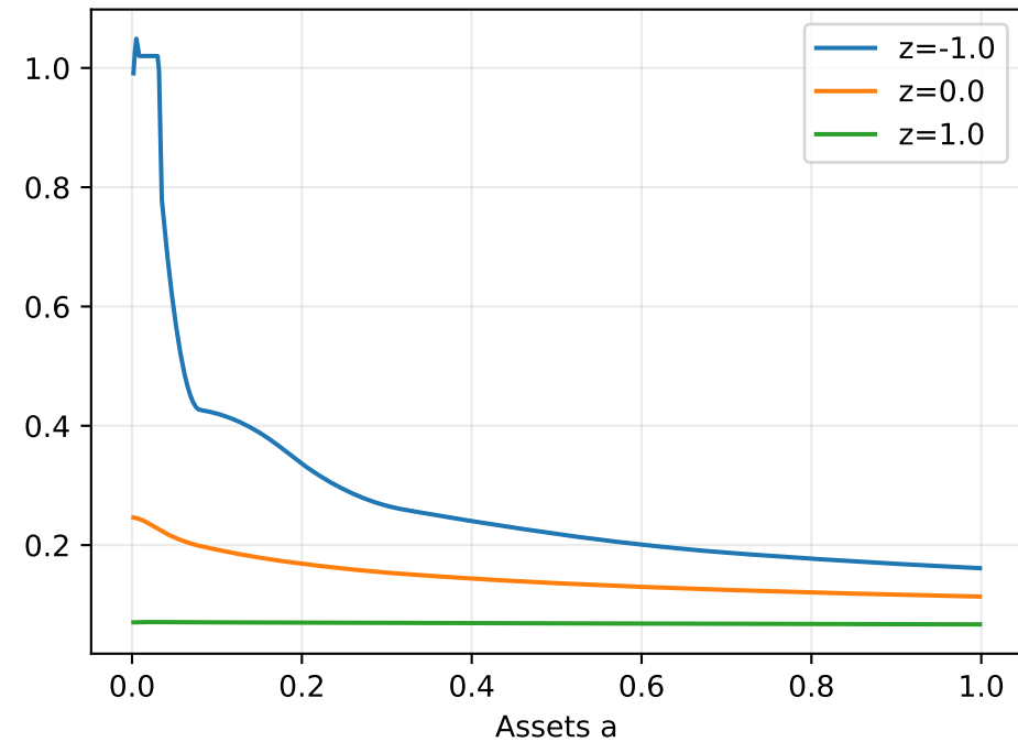
MPC dc/da (spline-smooth)
