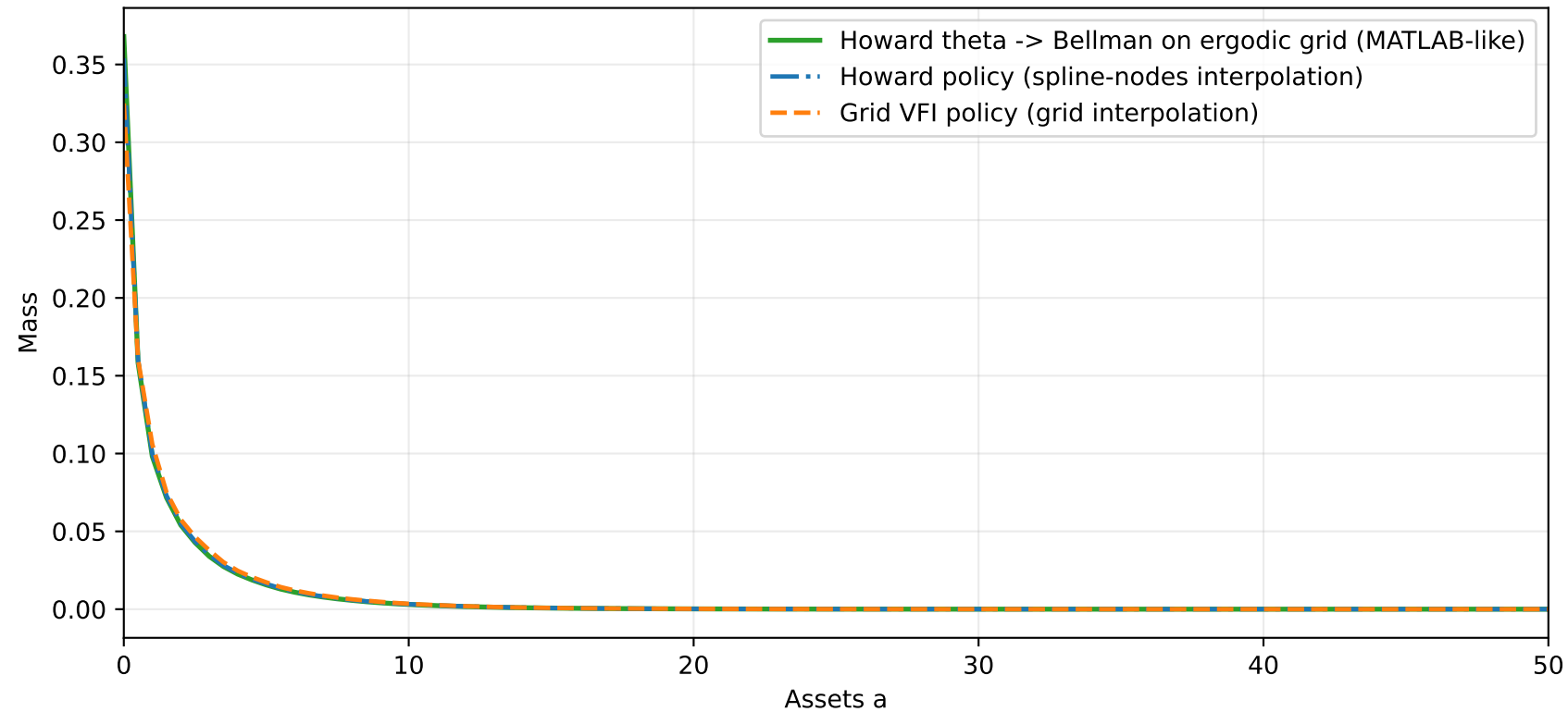
Ergodic marginal distribution over assets: policy discretization comparison
