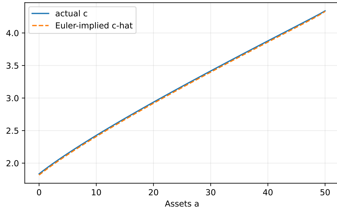
Consumption: actual vs Euler (z=1.049, collocation nodes)
