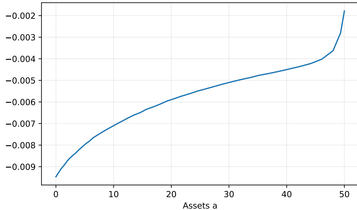
Euler error (c-hat - c)/c at collocation nodes
