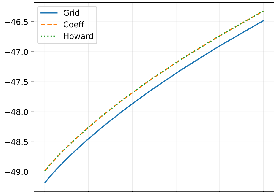
Savings, z=-1.0
