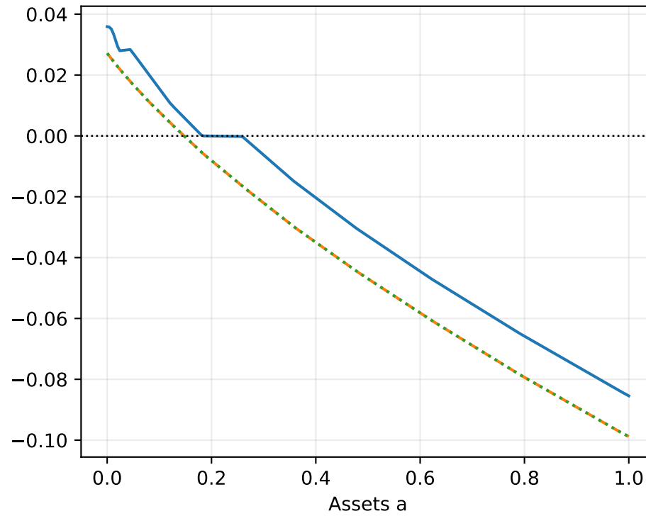
Savings, z=0.0
