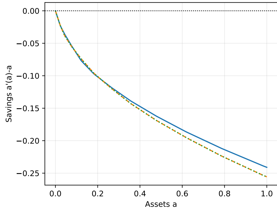
Savings, z=-1.0
