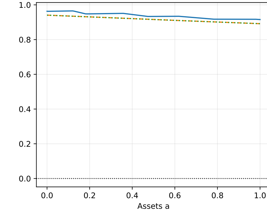
Savings, z=1.0
