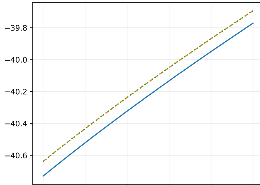
Savings, z=0.0
