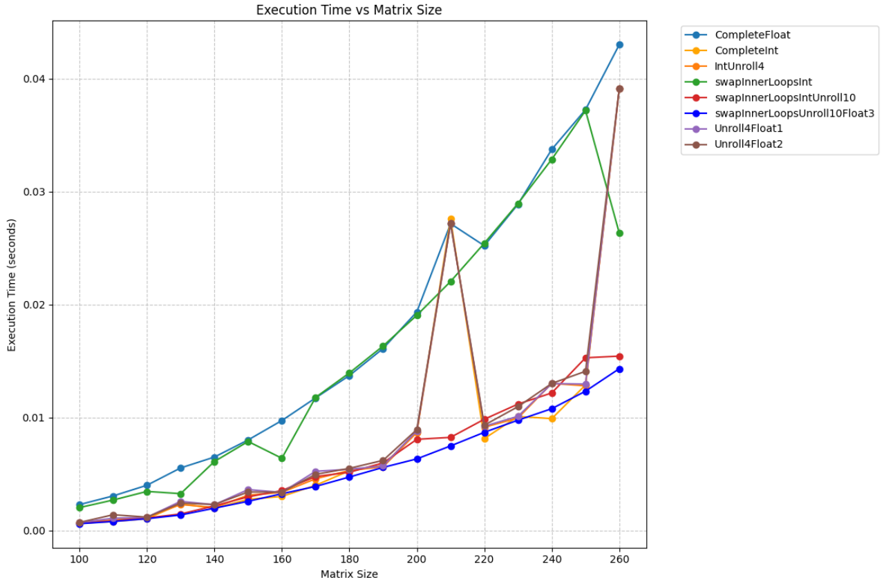
Figure 5: Execution Time vs Matrix Size for all versions
