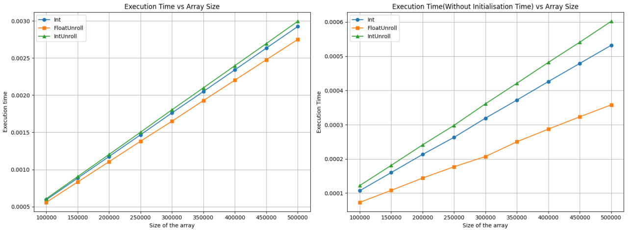
Figure 6: Execution Time vs Array Size
