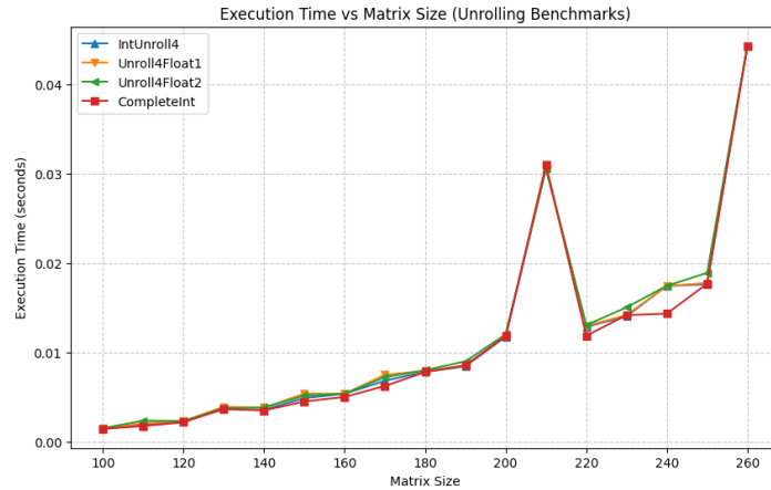
Figure 2: Execution Time vs Matrix Size for programs with Unrolling by factor 4
