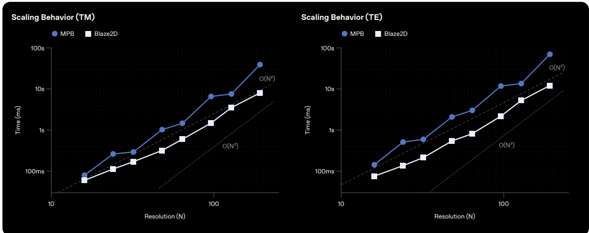
Figure 14: The same data on log-log axes with power-law fits, which makes the two solvers' scaling exponents directly comparable.
