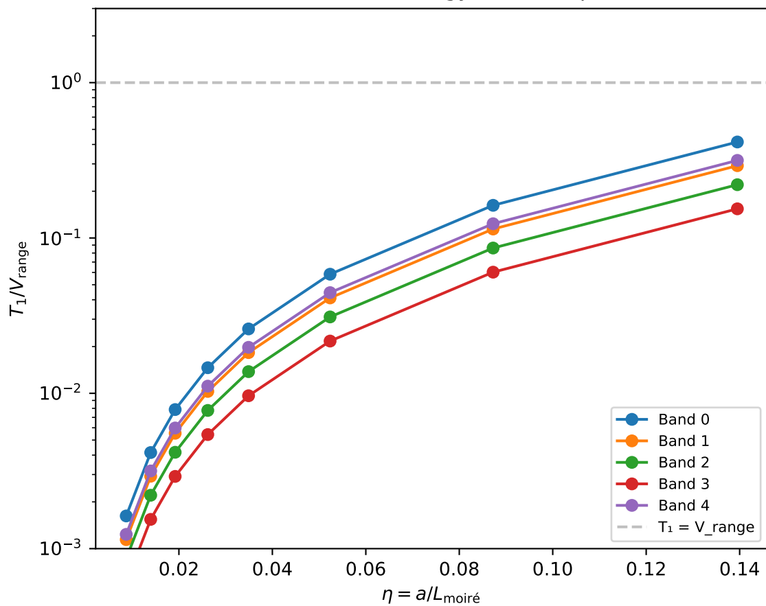
(c) Kinetic energy scale vs \eta
