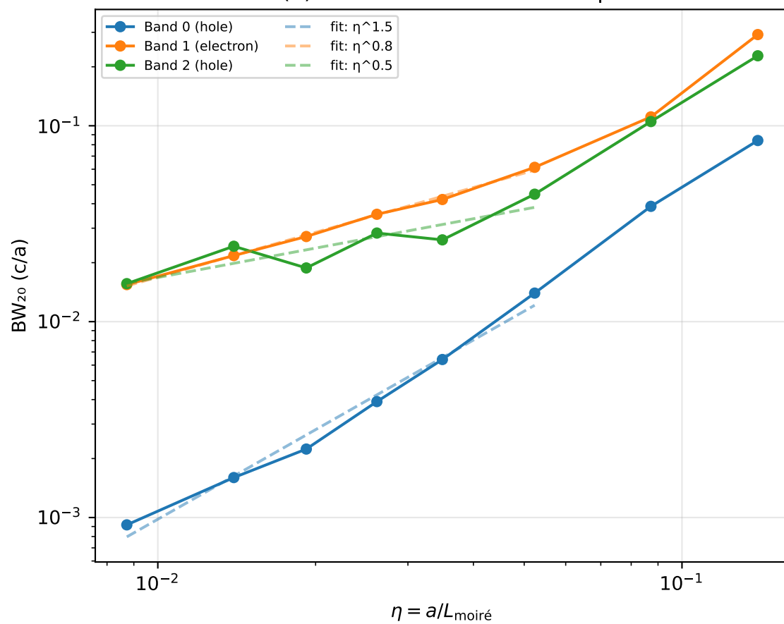
(c) Kinetic energy scale
