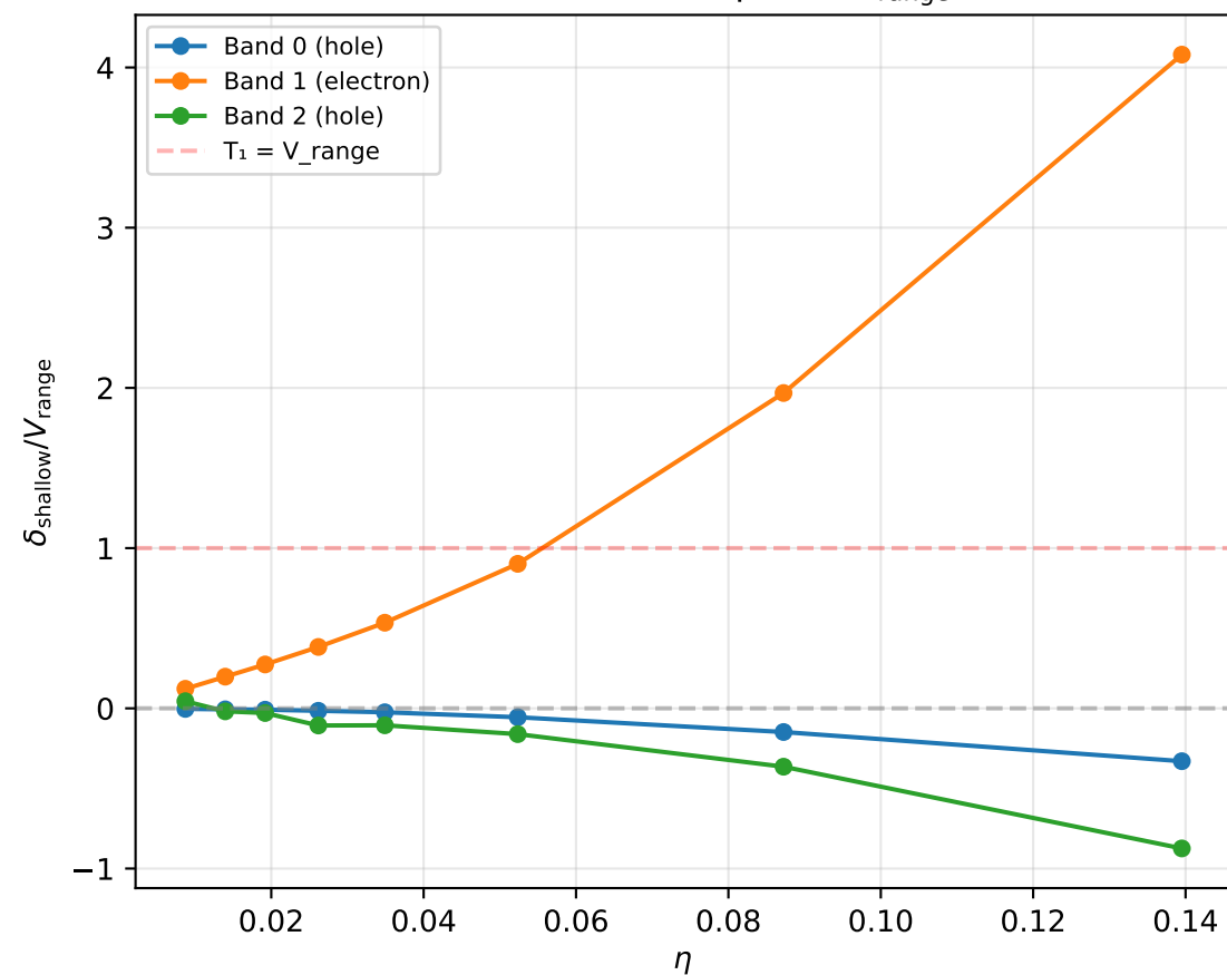
(b) Bound state depth ( \delta/V_{\text{range}} )
