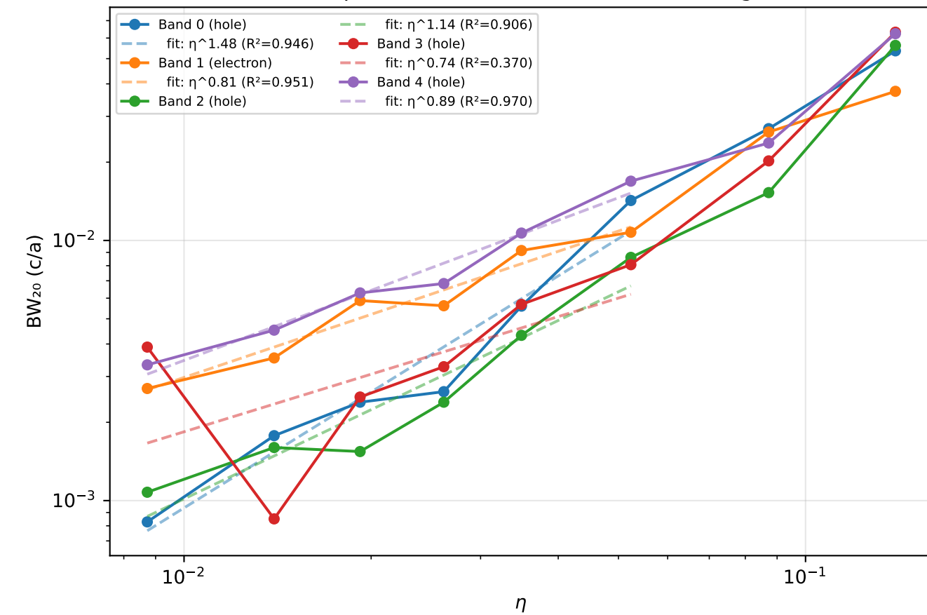
(c) Option B: miniband bandwidth scaling
