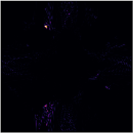
M10: B0(53%) \lambda=0.13049
