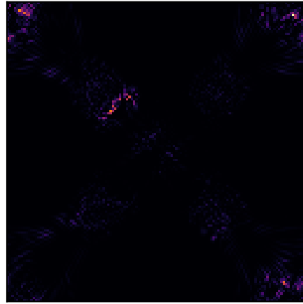
M8: B4(98%) \lambda=0.13046
