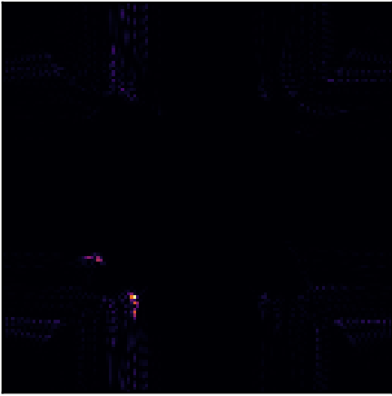
M7: B0(98%) \lambda=0.13043
