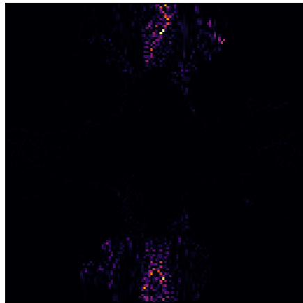
M19: B3(100%) \lambda=0.13065
