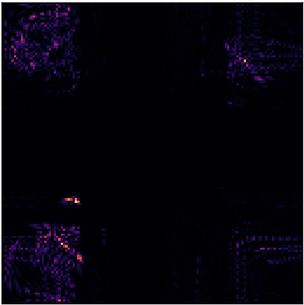
M15: B3(98%) \lambda=0.13061
