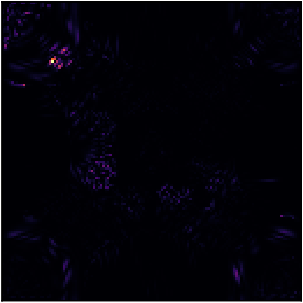
M5: B3(99%) \lambda=0.13039
