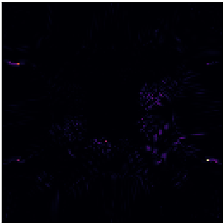
M16: B4(99%) \lambda=0.13063
