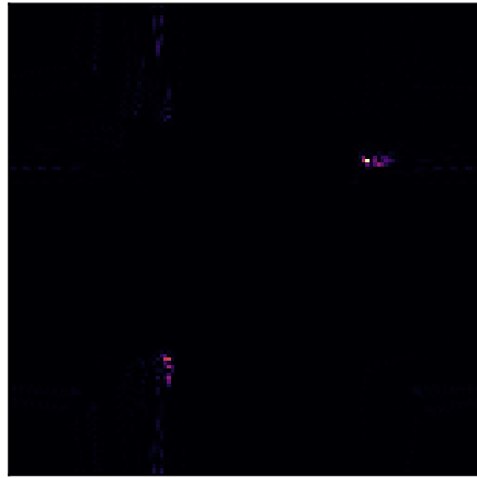
M14: B2(100%) \lambda=0.13058
