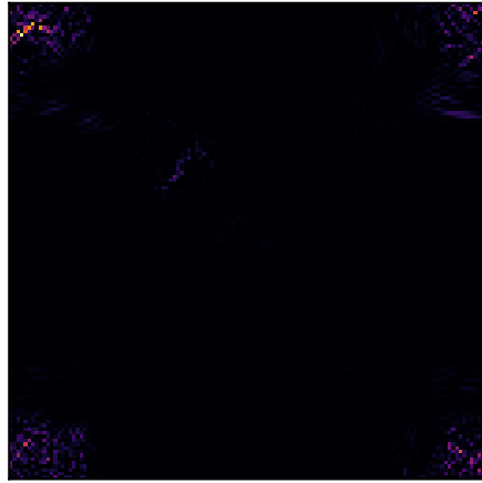
M9: B1(98%) \lambda=0.13046
