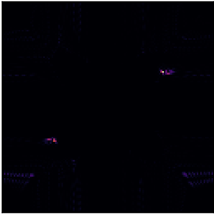
M11: B3(36%) \lambda=0.13049
