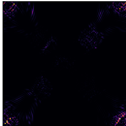
M18: B2(99%) \lambda=0.13064
