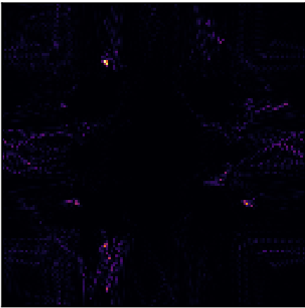
M17: B1(99%) \lambda=0.13063
