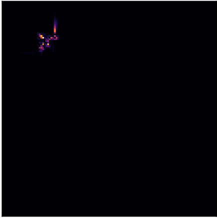
M6: B1(99%) \lambda=0.13042
