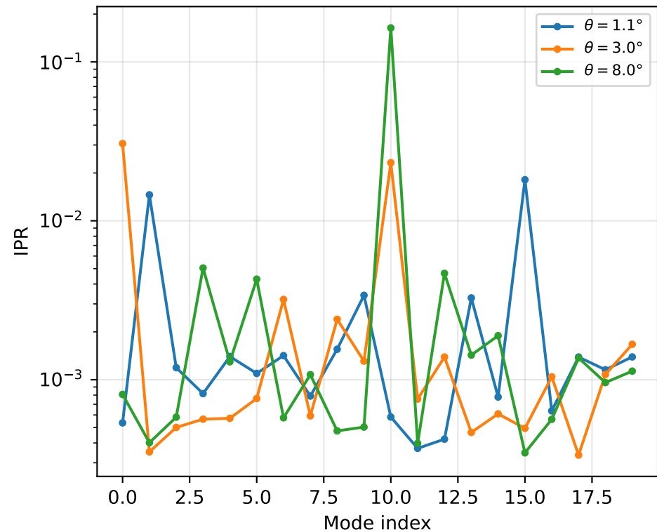
Inverse Participation Ratio
