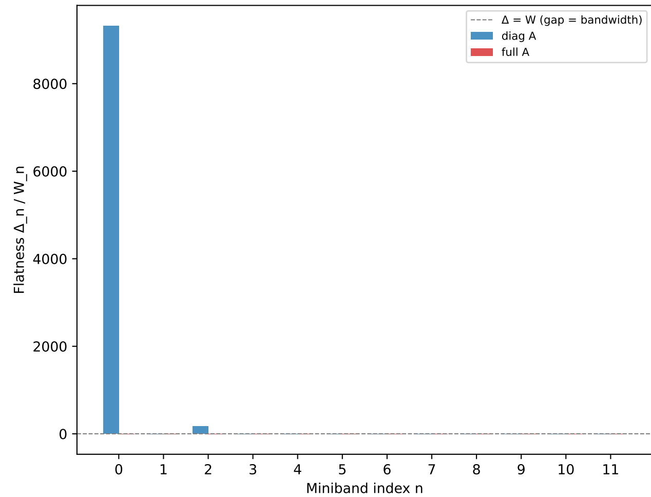
(d) Flatness ratio ( \Delta/W > 1 = isolated flat band)
