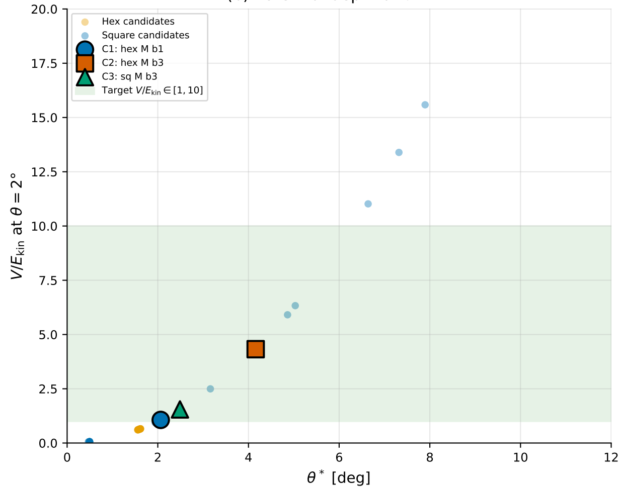
(b) Potential depth at \theta = 2^\circ
