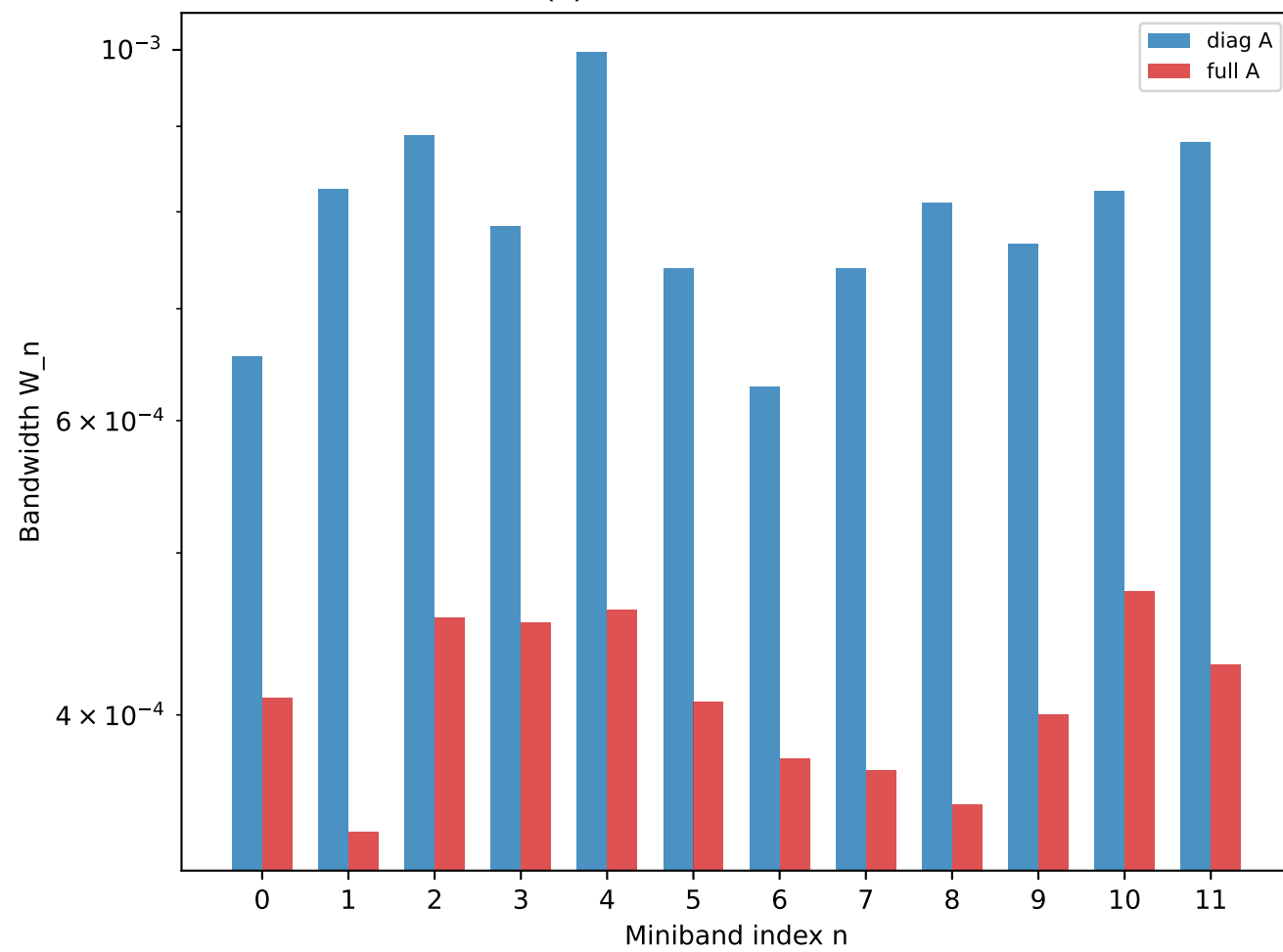
(c) Miniband bandwidths
