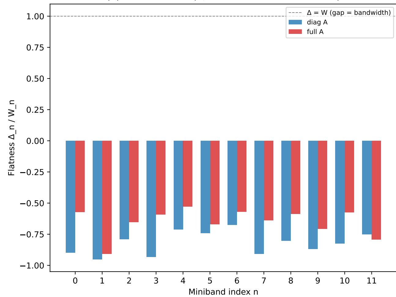
(d) Flatness ratio ( \Delta/W > 1 = isolated flat band)
