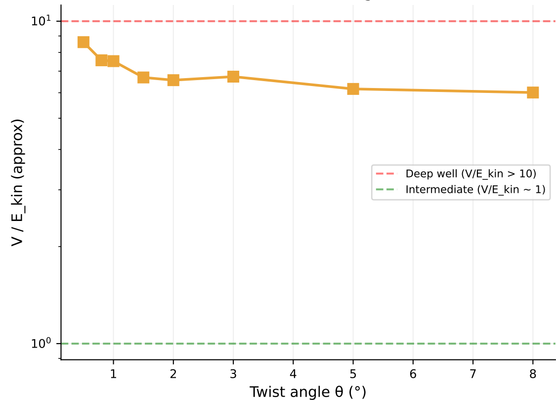
(b) Confinement regime
