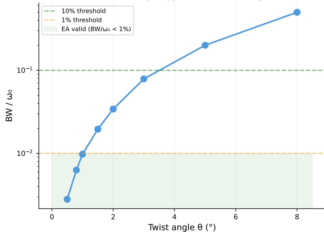
(a) Envelope approximation validity
