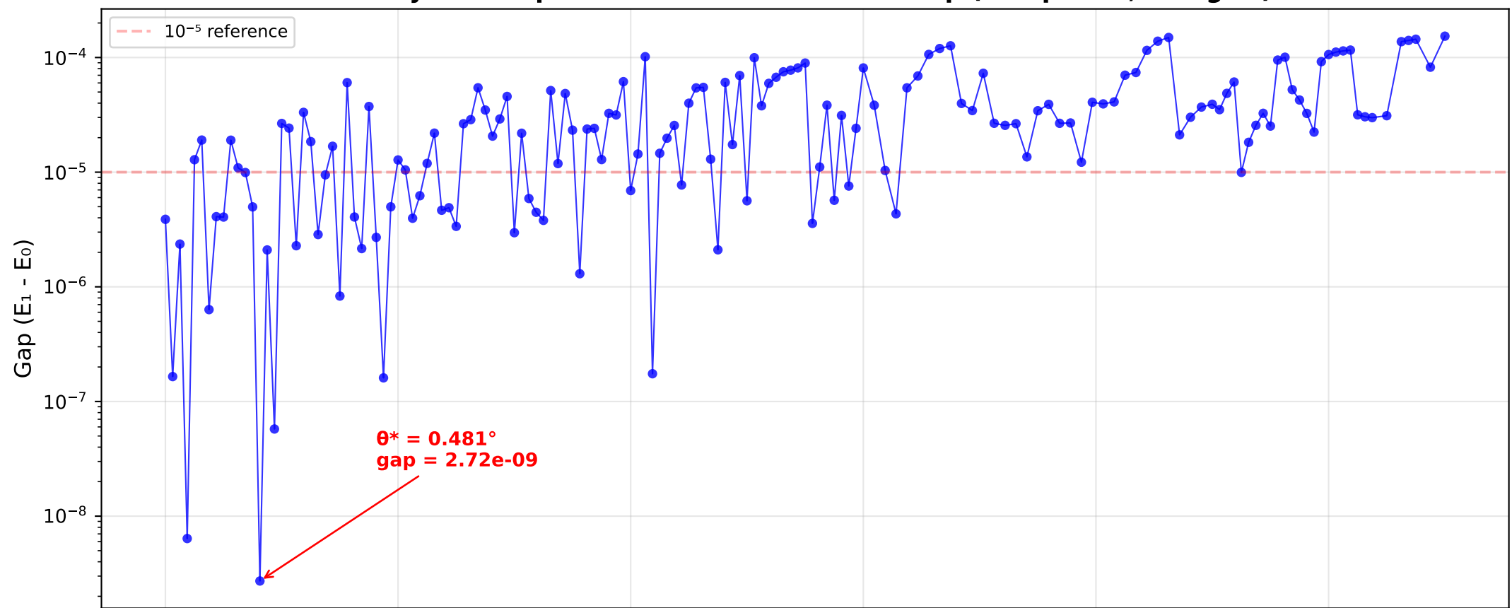
Honeycomb K-point Moiré — Bisection Sweep (157 points, 128 grid)
