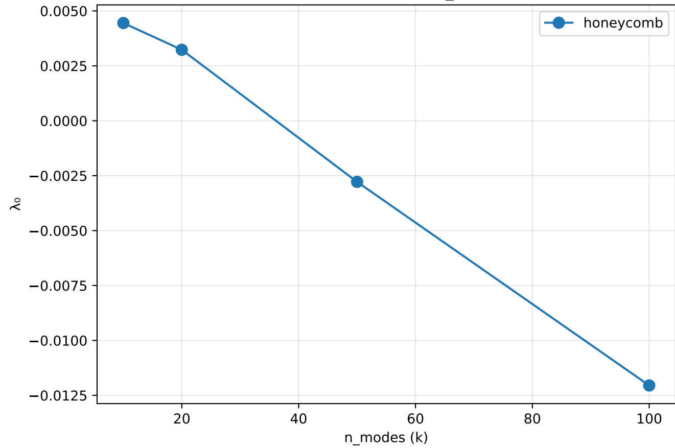
Ground state \lambda_0 vs n_{\text{modes}}
