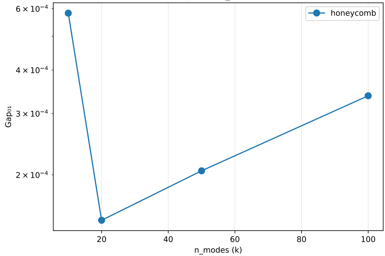
Gap 01 vs n_{\text{modes}}
