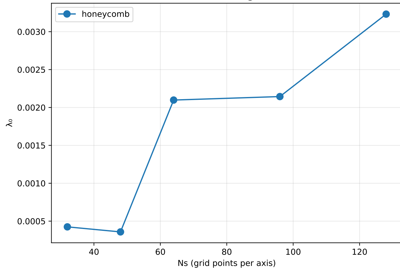
Ground state \lambda_0 vs grid size N_s
