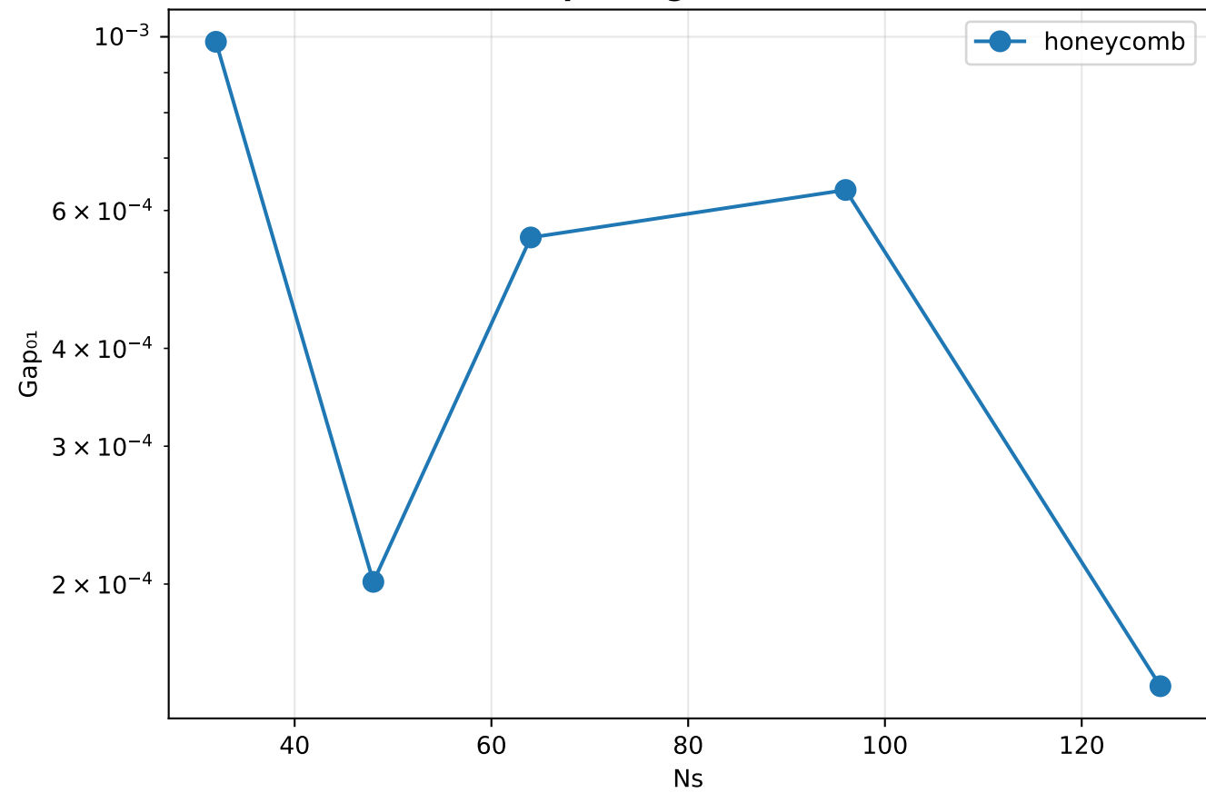
Gap 01 vs grid size N_s
