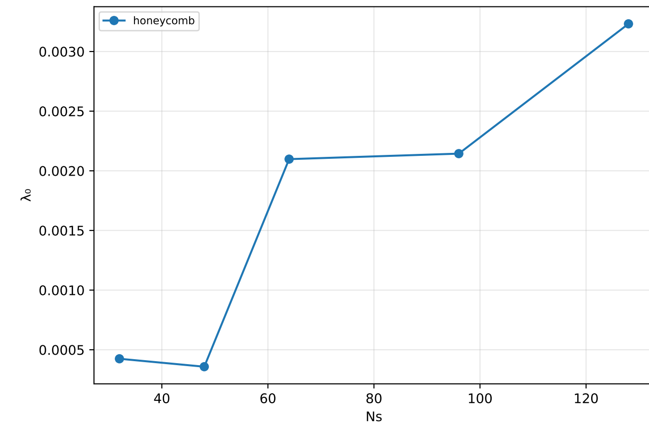
\lambda_0 vs N_s
