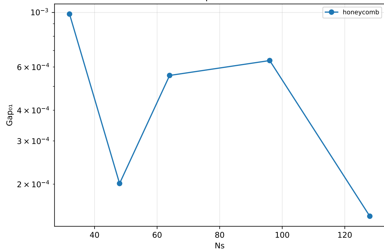
Gap 01 vs N_s
