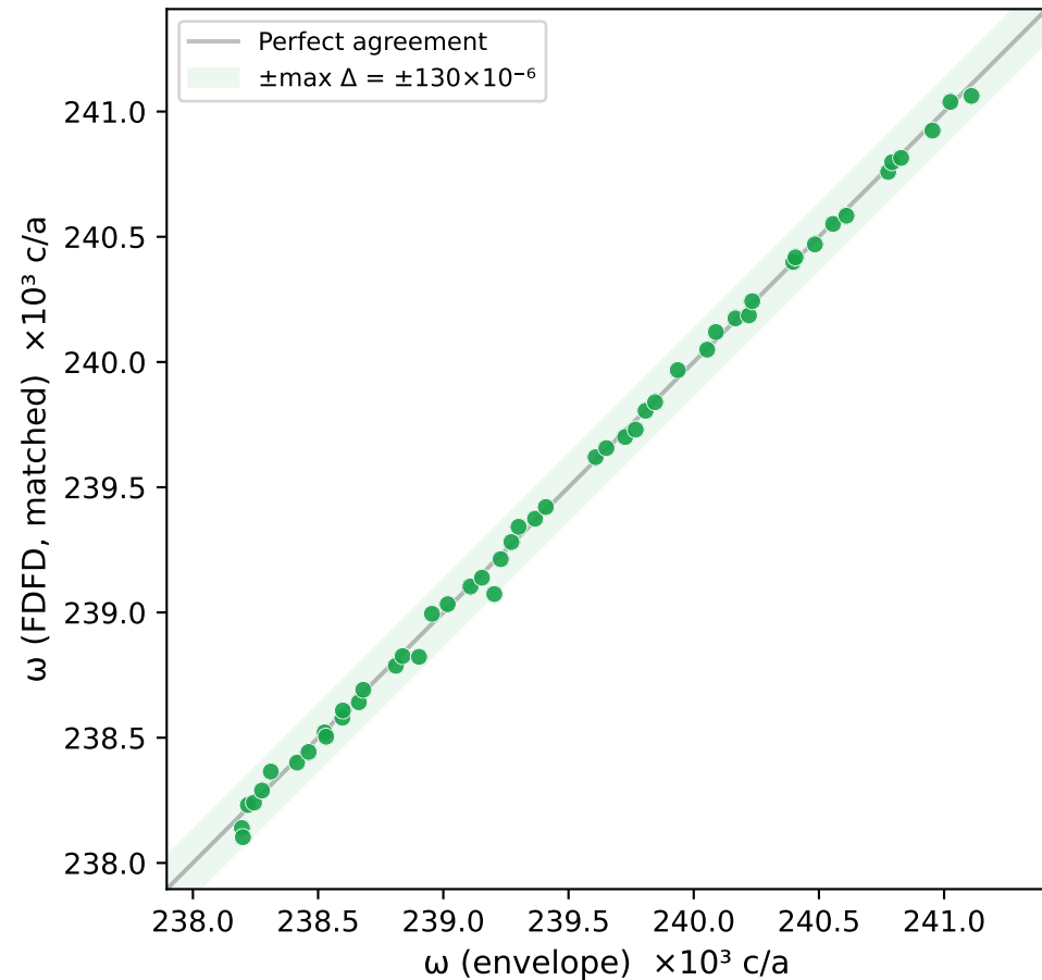
(a) Frequency agreement
