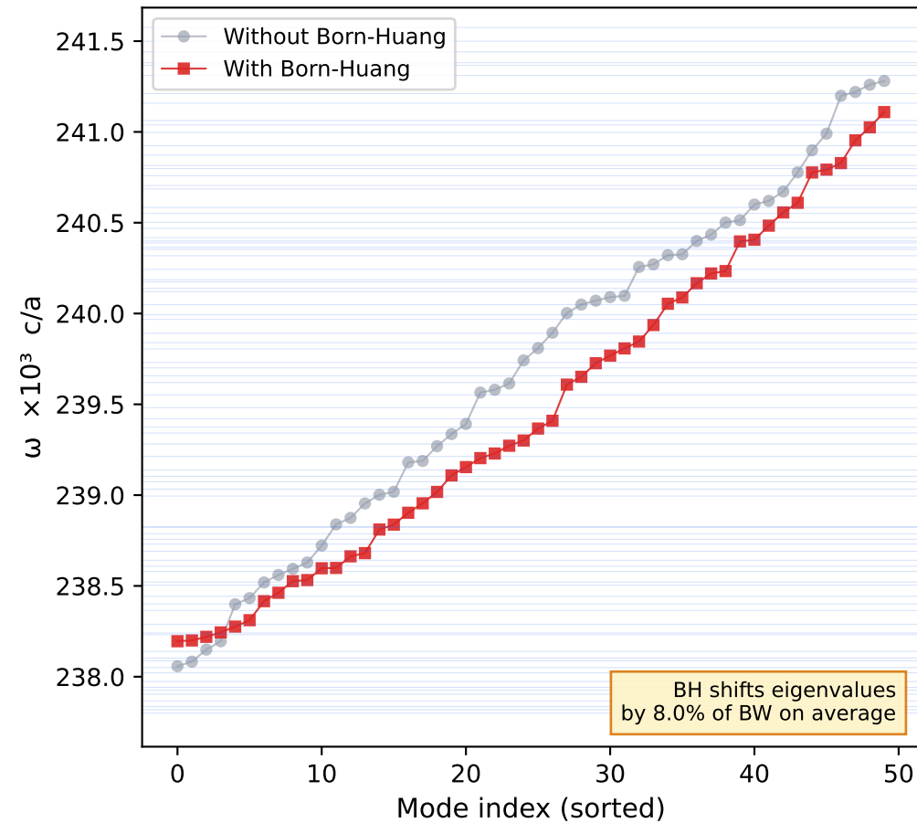
(c) Born-Huang correction
