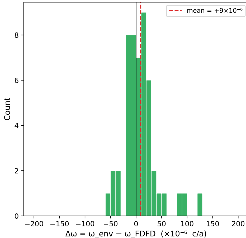
(b) Residual distribution
