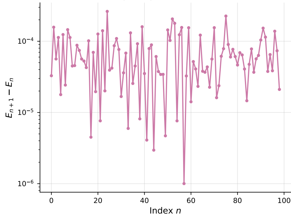
(b) Level spacings (median=0.000056)
