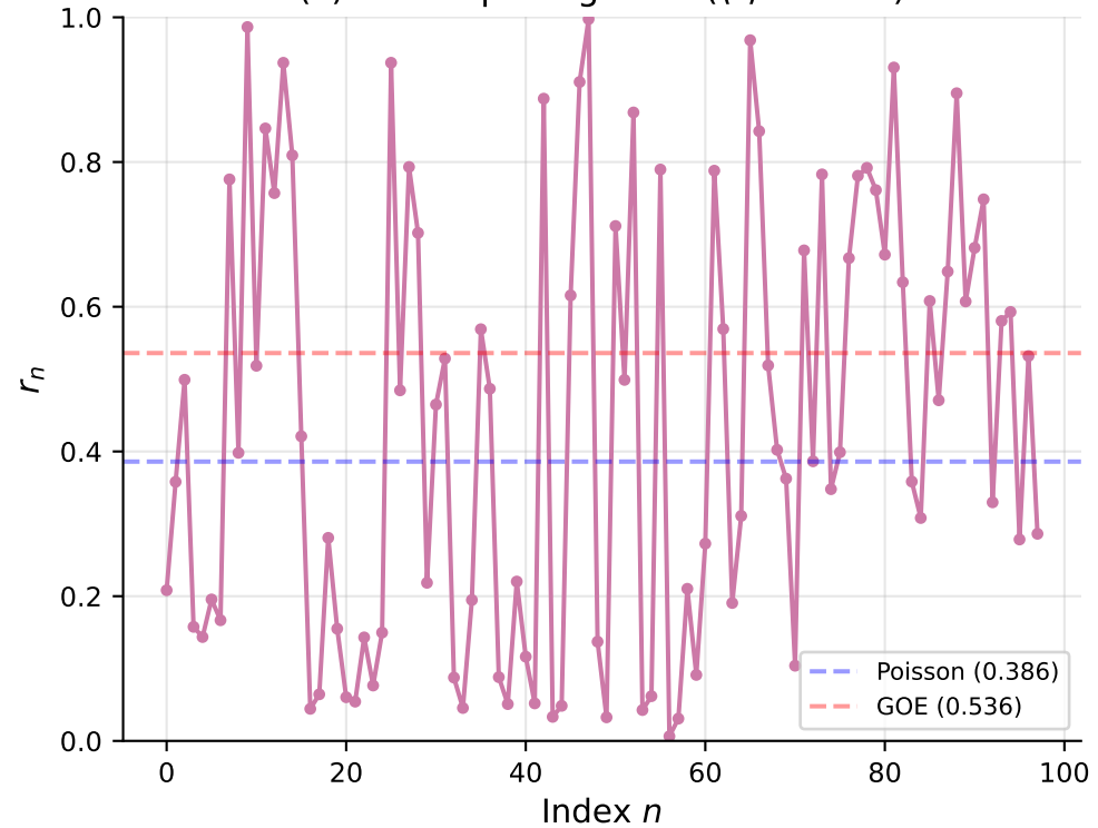
(c) Level spacing ratio ( \langle r \rangle = 0.442 )
