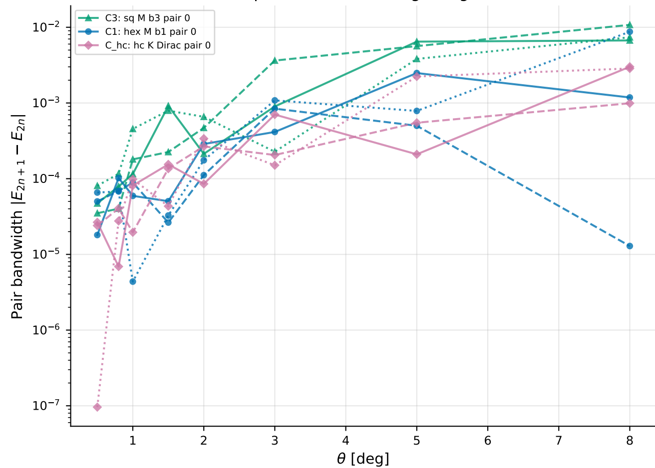
(b) Band-pair bandwidth (magic angle search)
