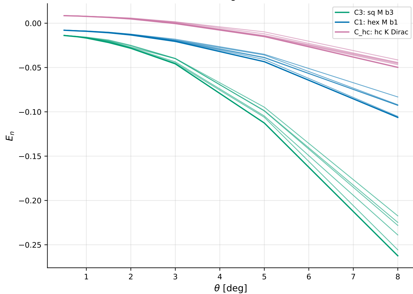
(a) Lowest 6 eigenvalues vs \theta
