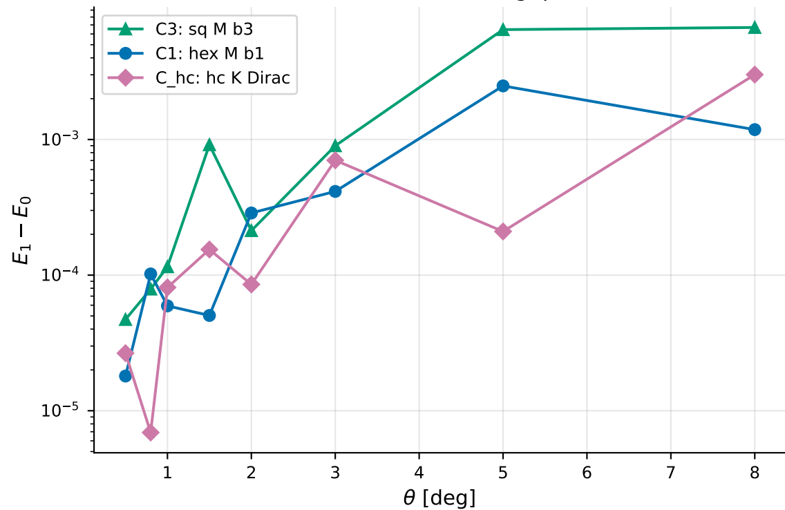
(b) Ground-state gap
