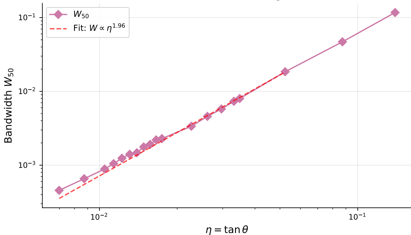
(b) Bandwidth scaling
