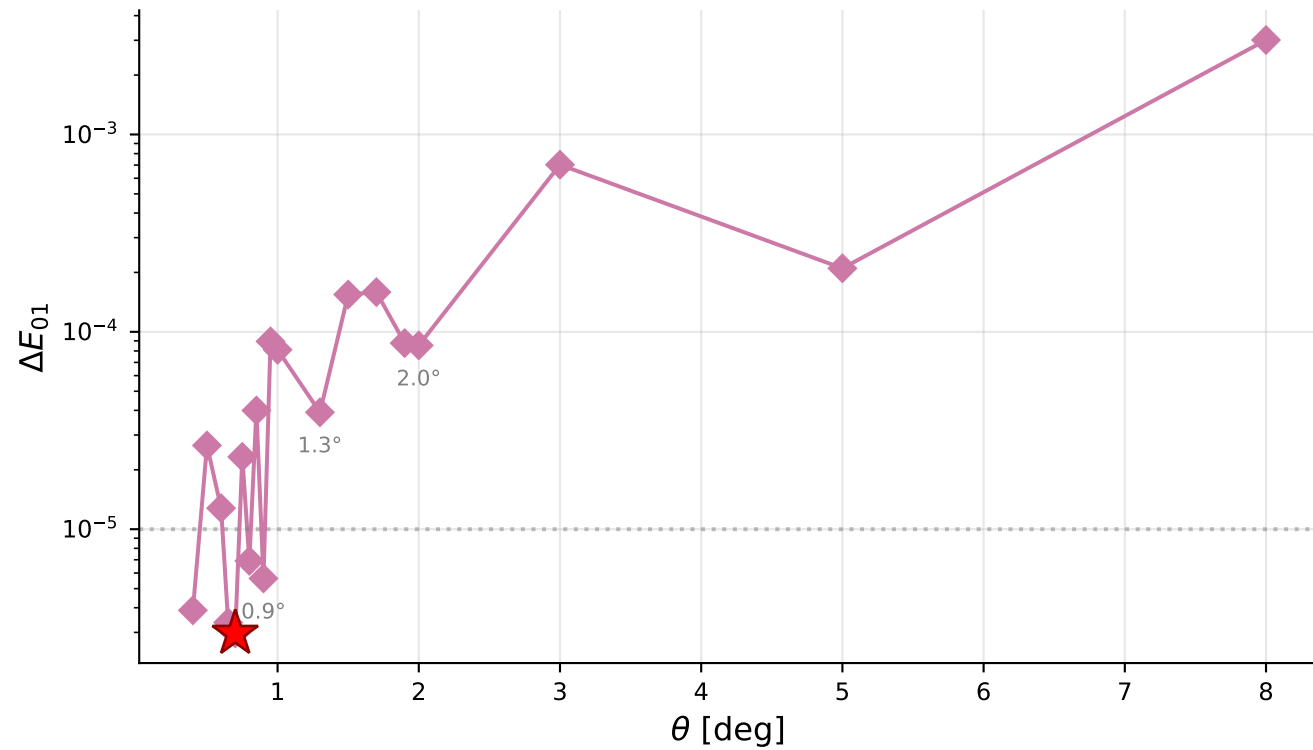
(a) Band gap E_1 - E_0 vs twist angle
