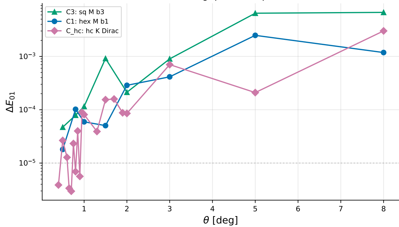
(b) Band gap (lowest pair)
