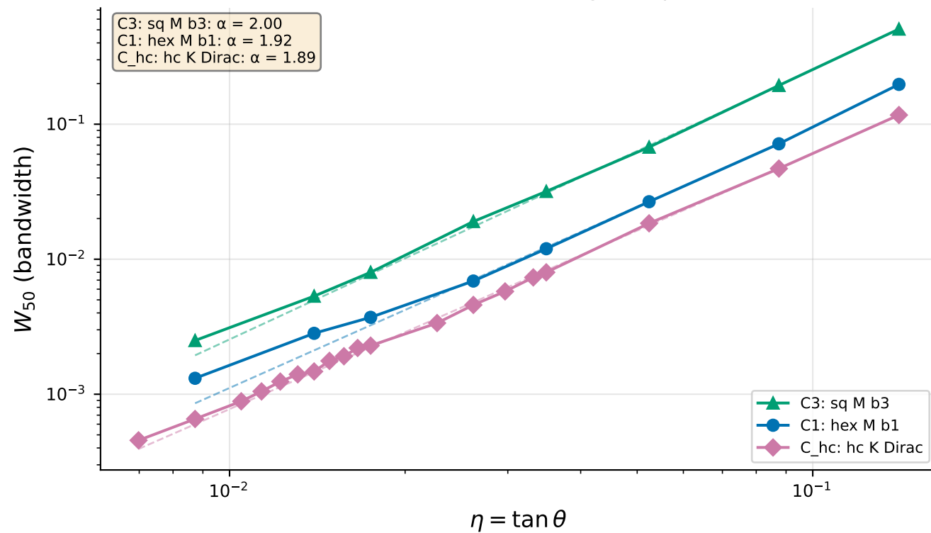
(a) Bandwidth scaling W \propto \eta^\alpha
