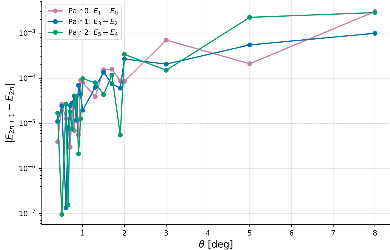
(b) Pair splittings (Dirac doublets)
