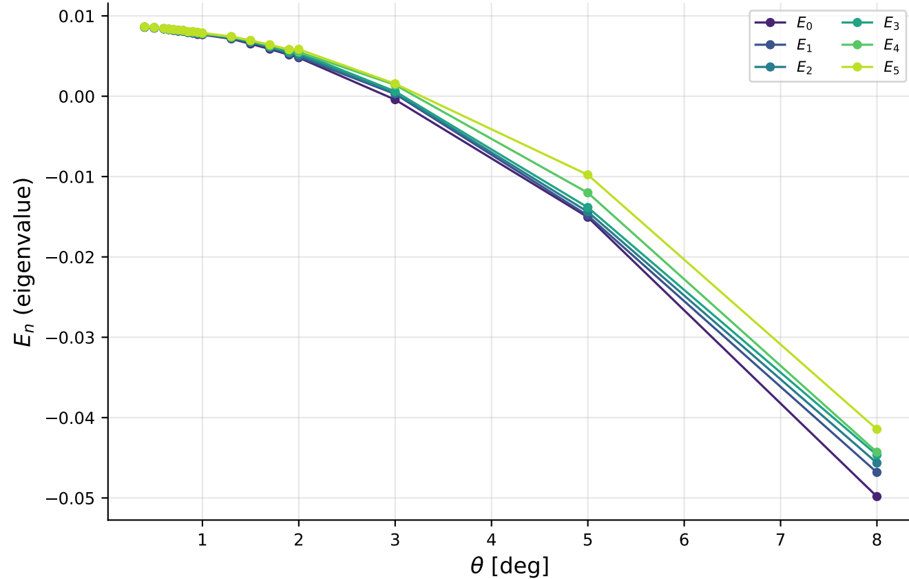
(a) Lowest 6 eigenvalues
