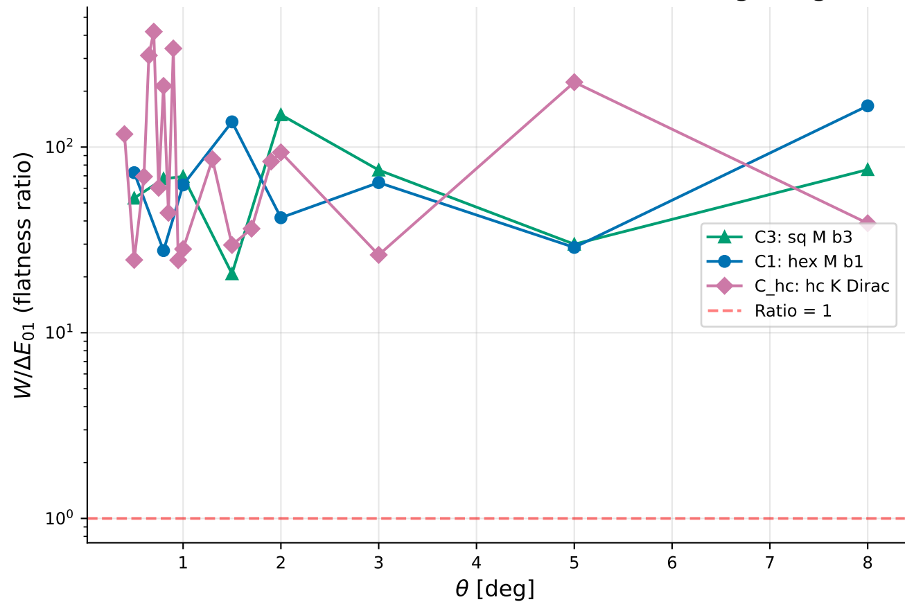
Flatness Ratio: Lower = Flatter Band (Better Magic Angle)
