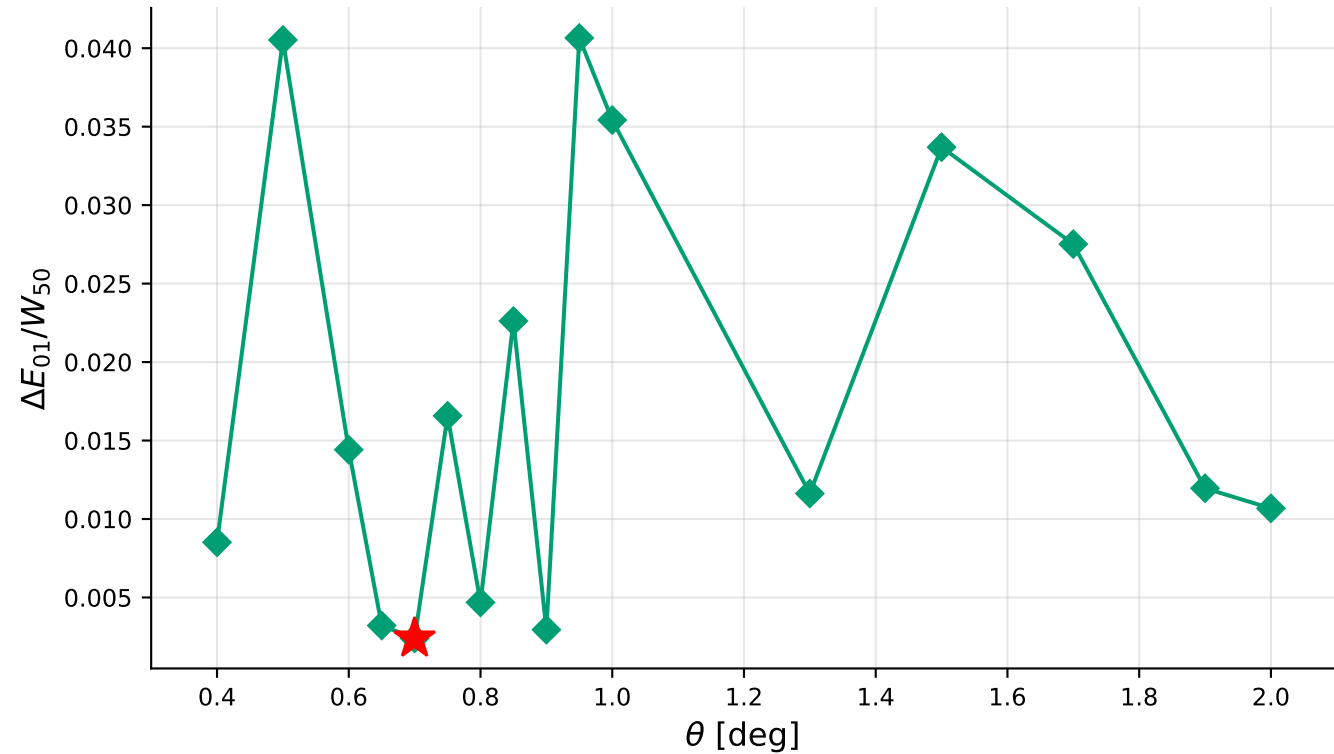
(b) Gap-to-bandwidth ratio
