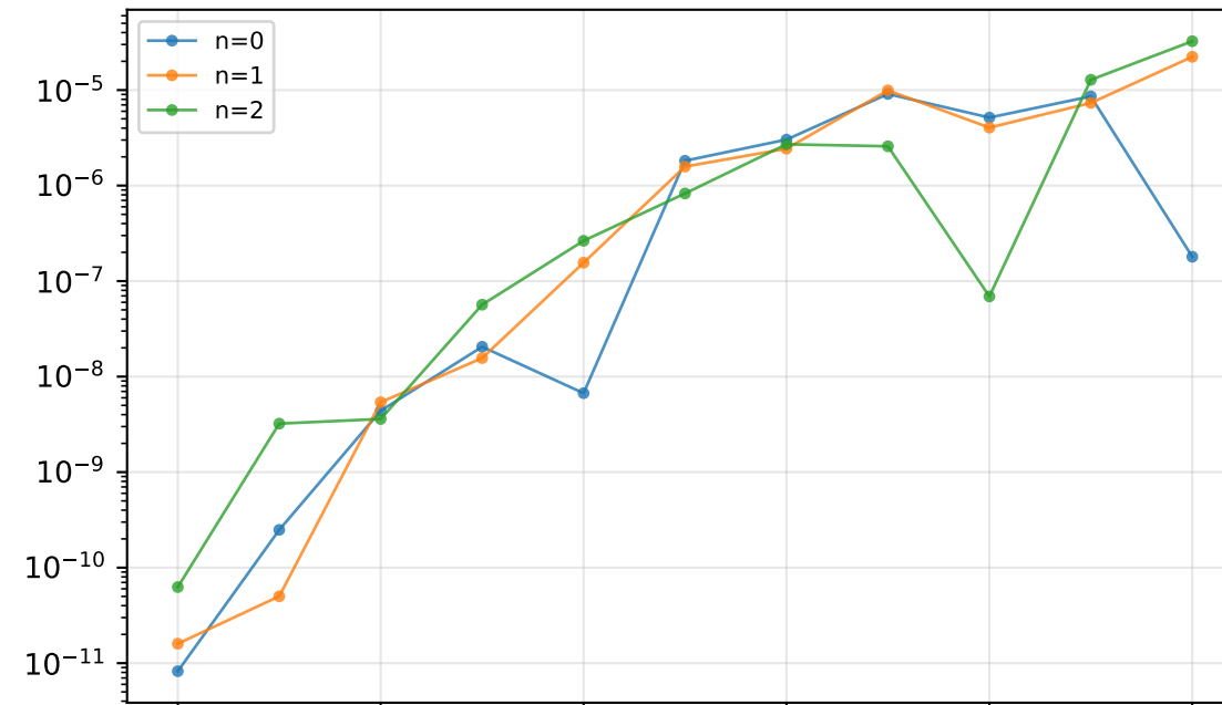
Honeycomb K-point
