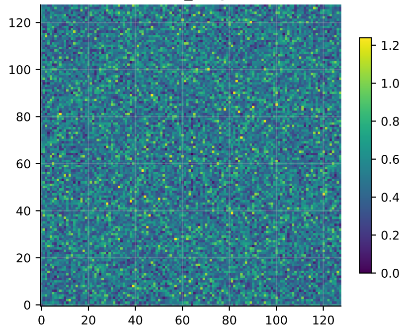
A_{01,\text{mag}}
