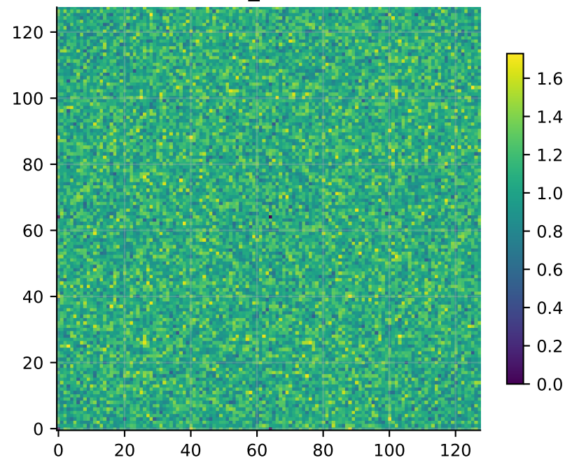
A_{01,\text{mag}}
