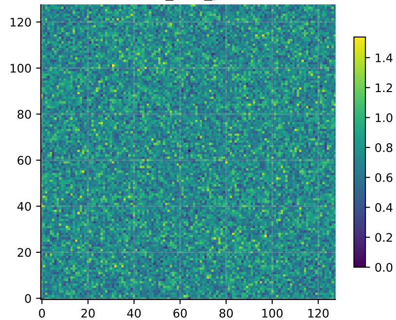
A_{\text{frob}_y}
