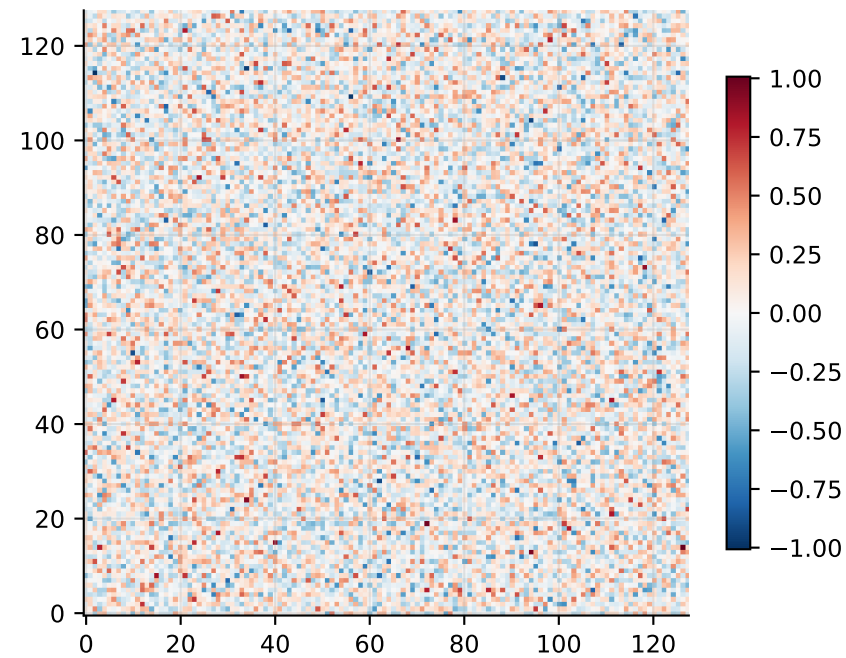
A_{\text{frob}_y}
