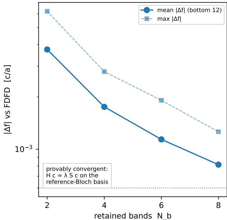
A Exact Galerkin model \rightarrow FDFD (7,1) \theta=16.3^\circ , variational, monotone
