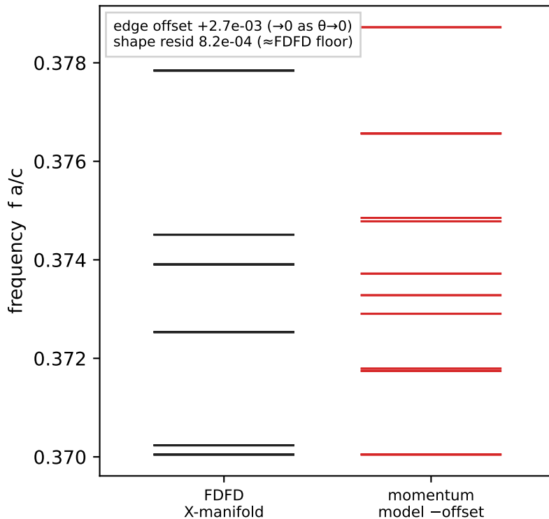
B Practical continuum model, 2^\circ (57,1): count 24/24, \times 4 quadruplets
