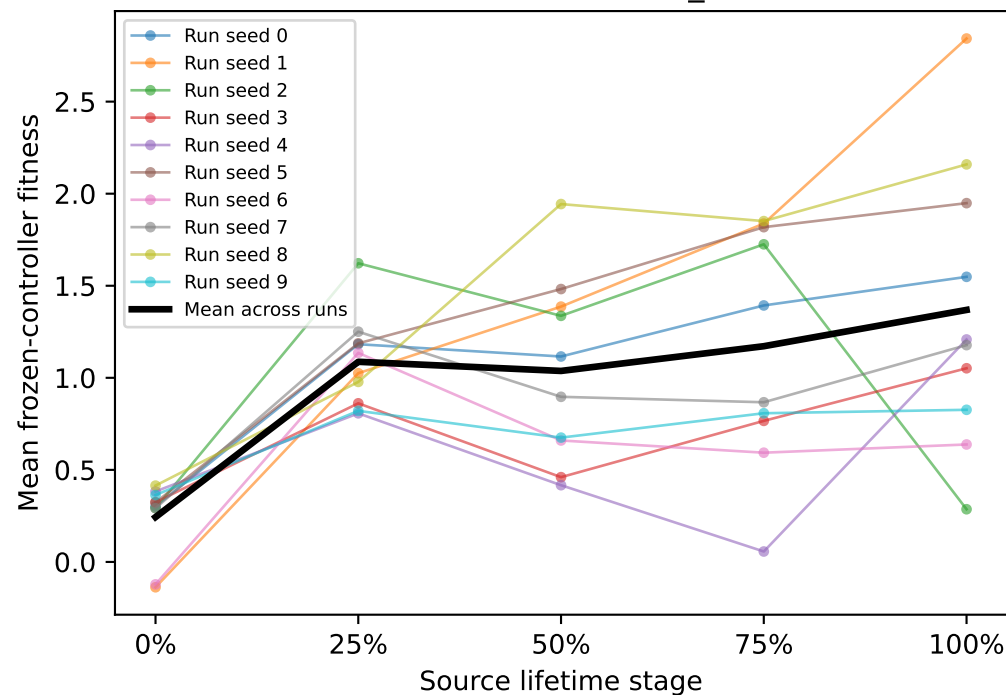
Thrower-v0 / thrower_arm
