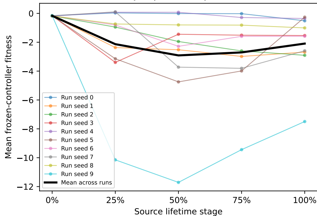
Thrower-v0 / thrower_arm
