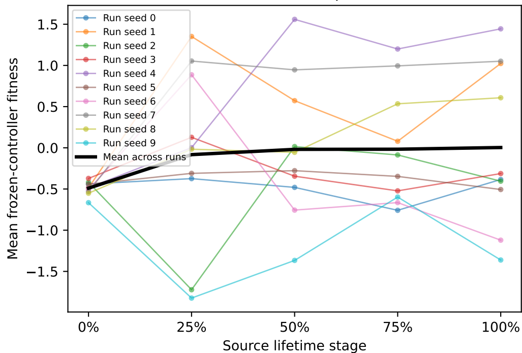
Thrower-v0 / biped
