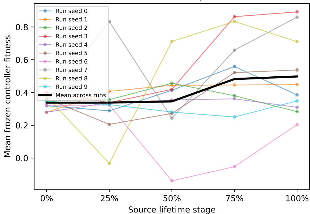
Walker-v0 / biped
